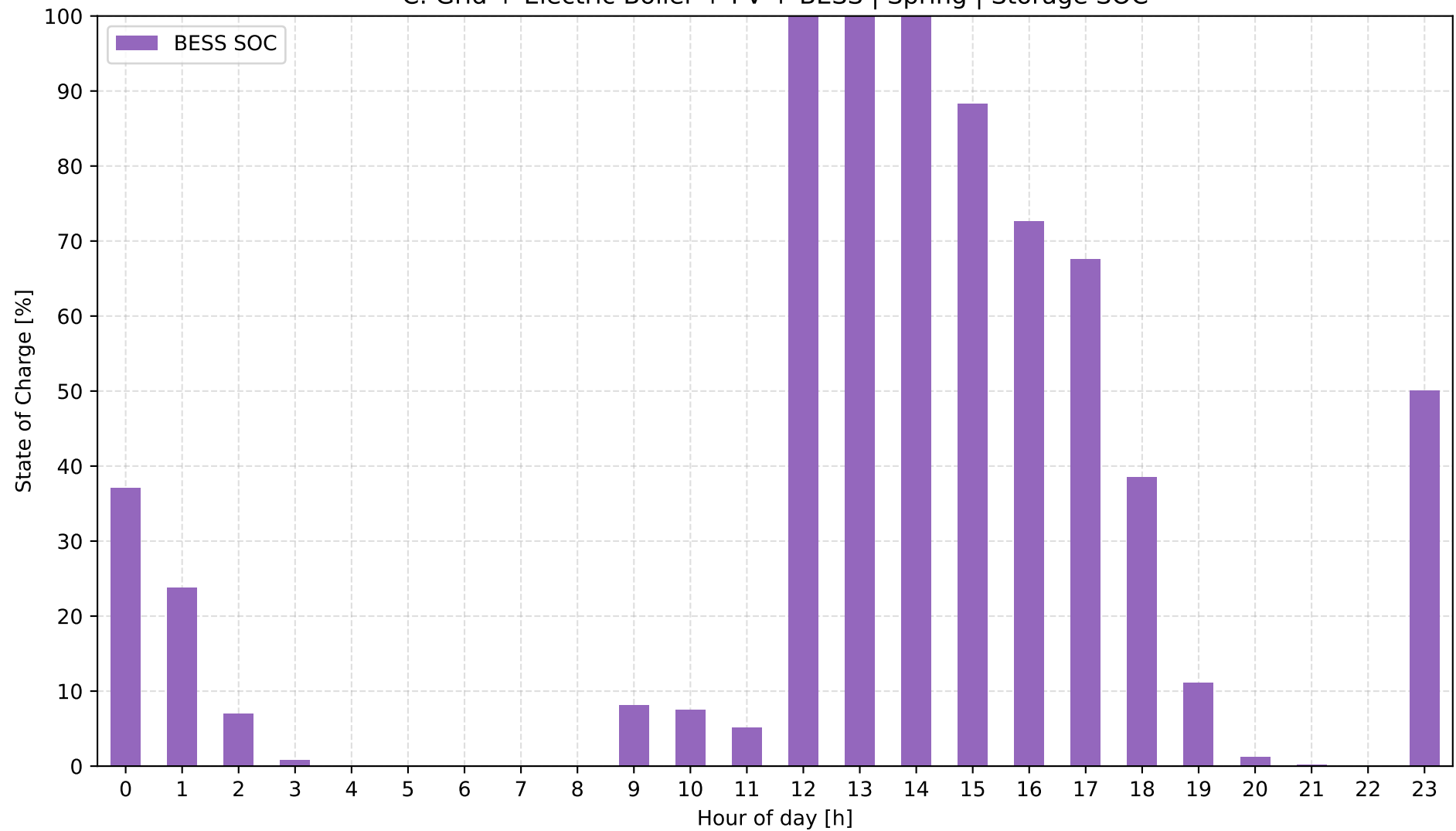
C: Grid + Electric Boiler + PV + BESS | Spring | Storage SOC
