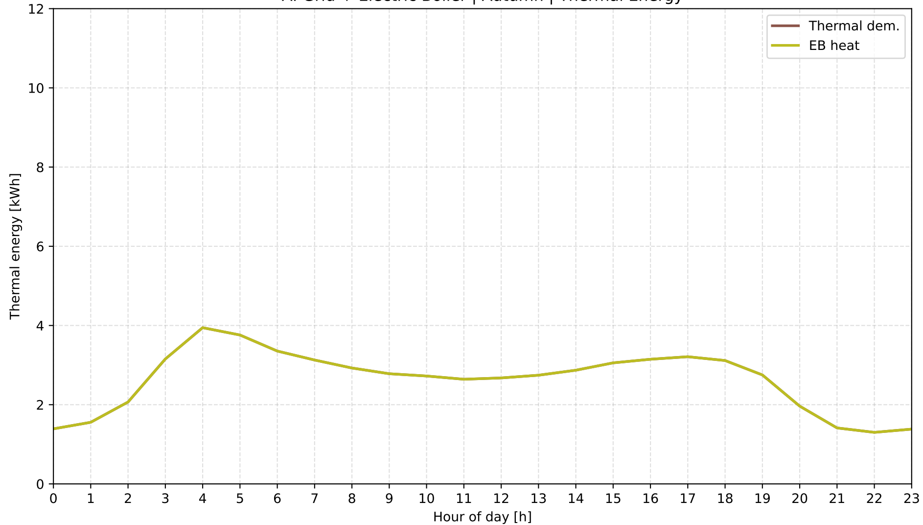
A: Grid + Electric Boiler | Autumn | Thermal Energy
