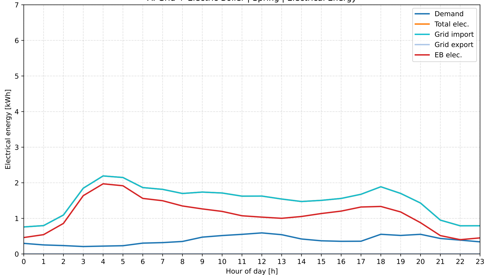
A: Grid + Electric Boiler | Spring | Electrical Energy
