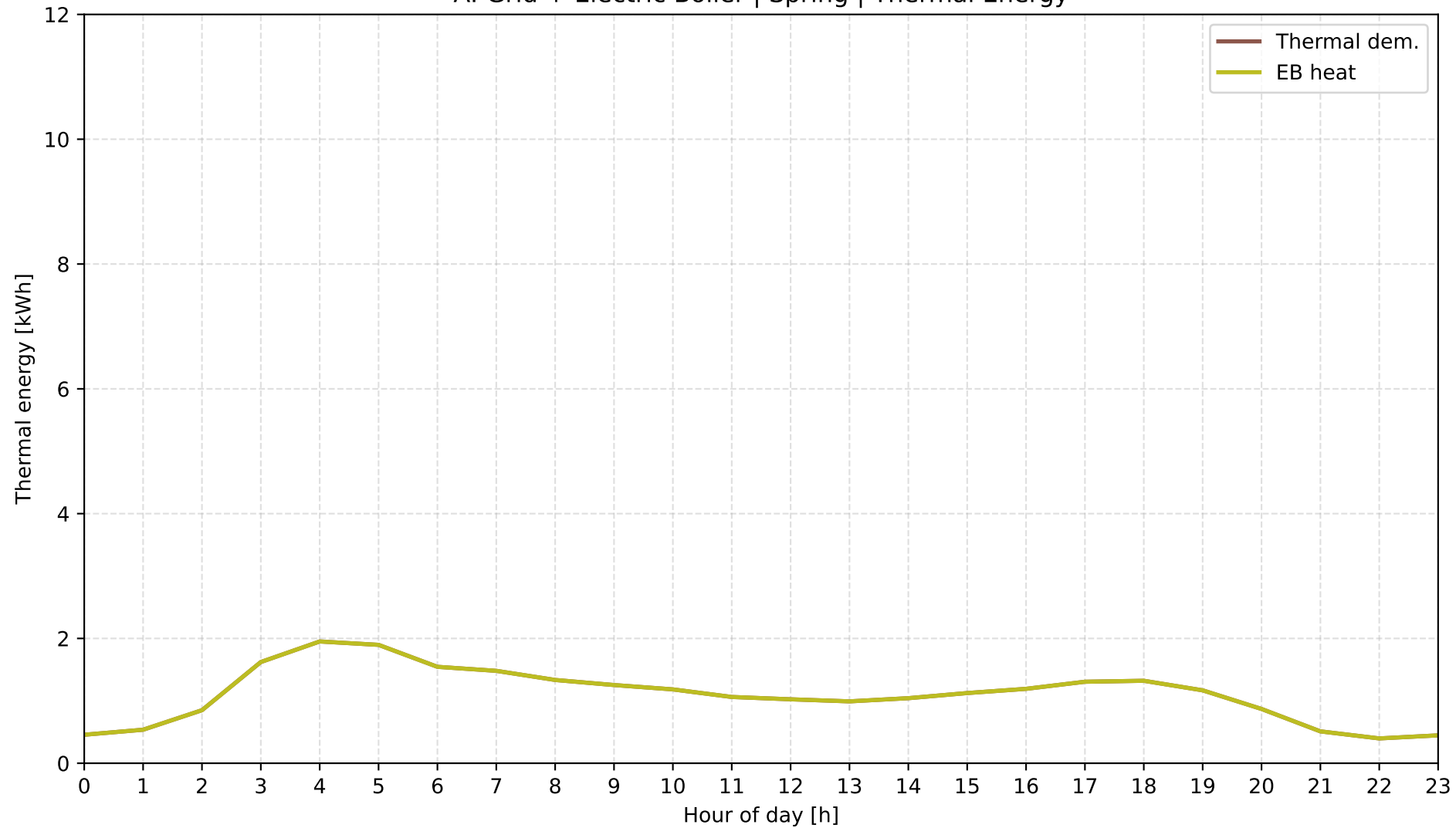
A: Grid + Electric Boiler | Spring | Thermal Energy
