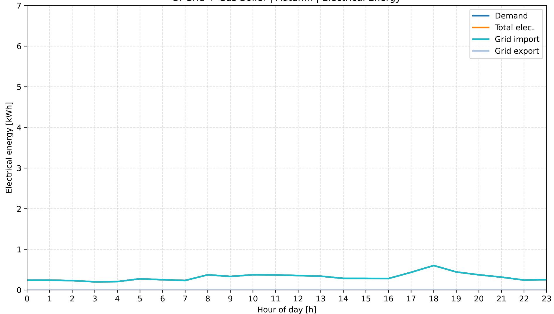
B: Grid + Gas Boiler | Autumn | Electrical Energy
