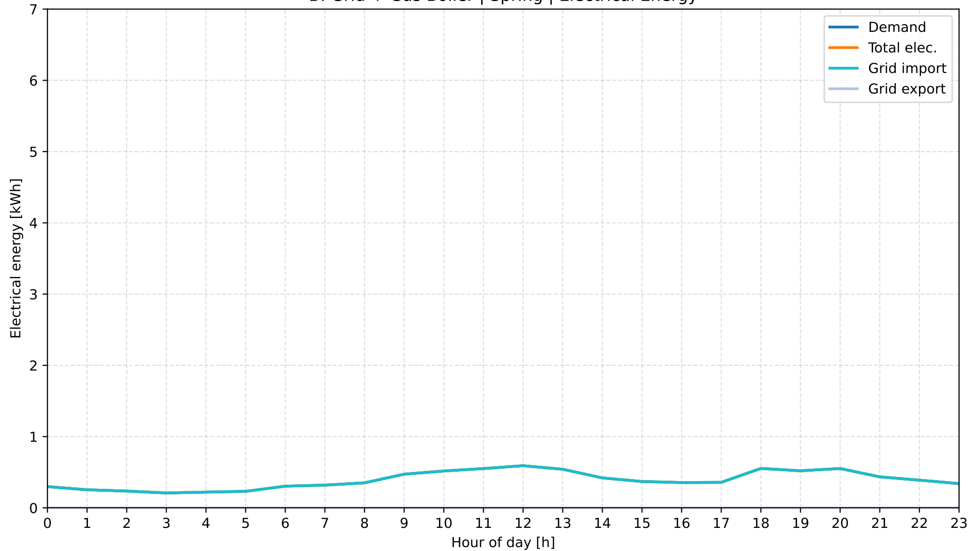
B: Grid + Gas Boiler | Spring | Electrical Energy
