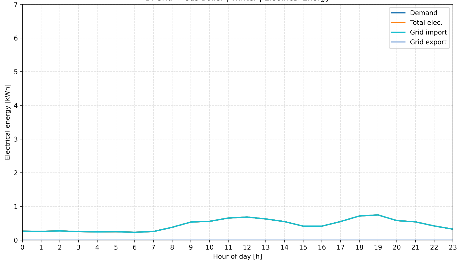
B: Grid + Gas Boiler | Winter | Electrical Energy
