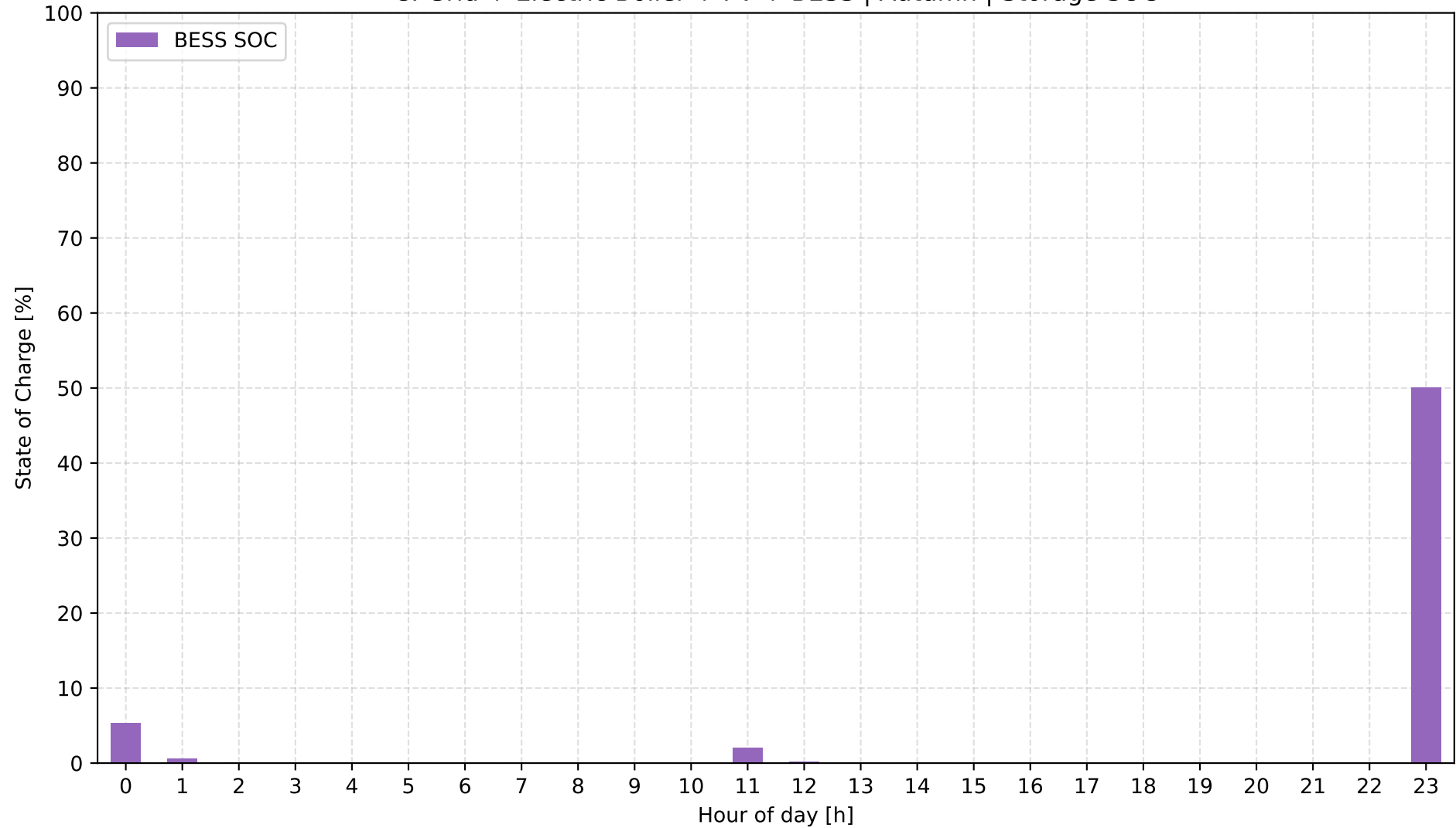
C: Grid + Electric Boiler + PV + BESS | Autumn | Storage SOC
