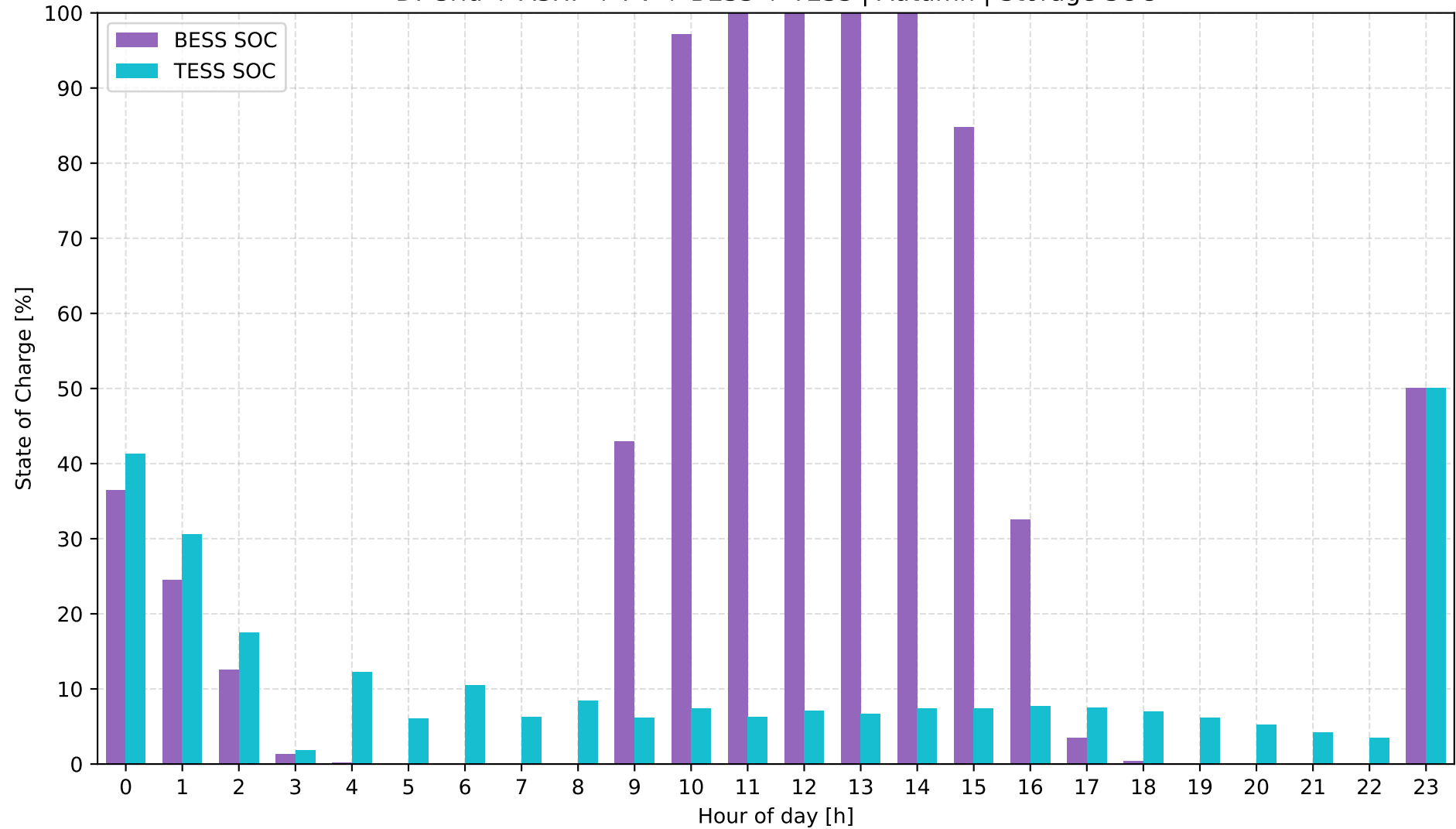
D: Grid + ASHP + PV + BESS + TESS | Autumn | Storage SOC
