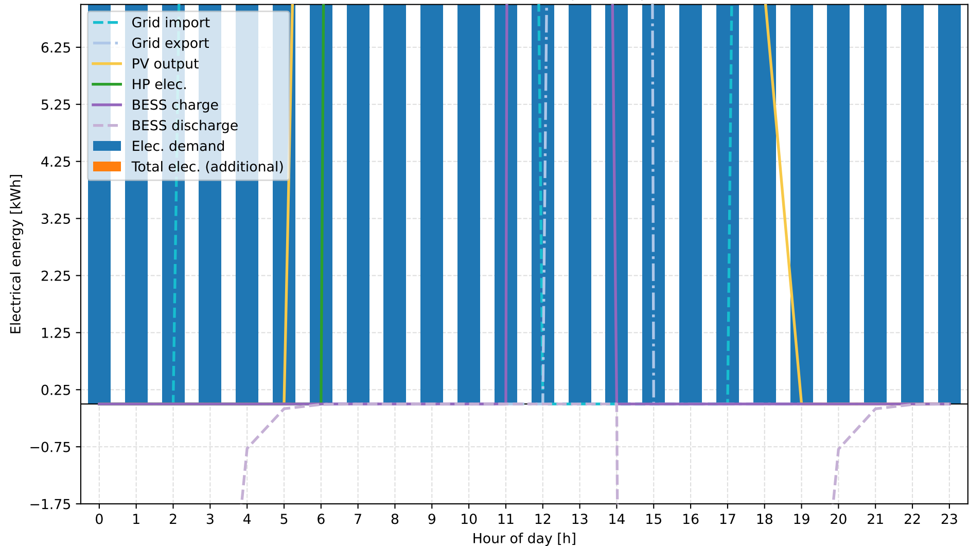
D: Grid + ASHP + PV + BESS + TESS | Spring | Electrical Energy
