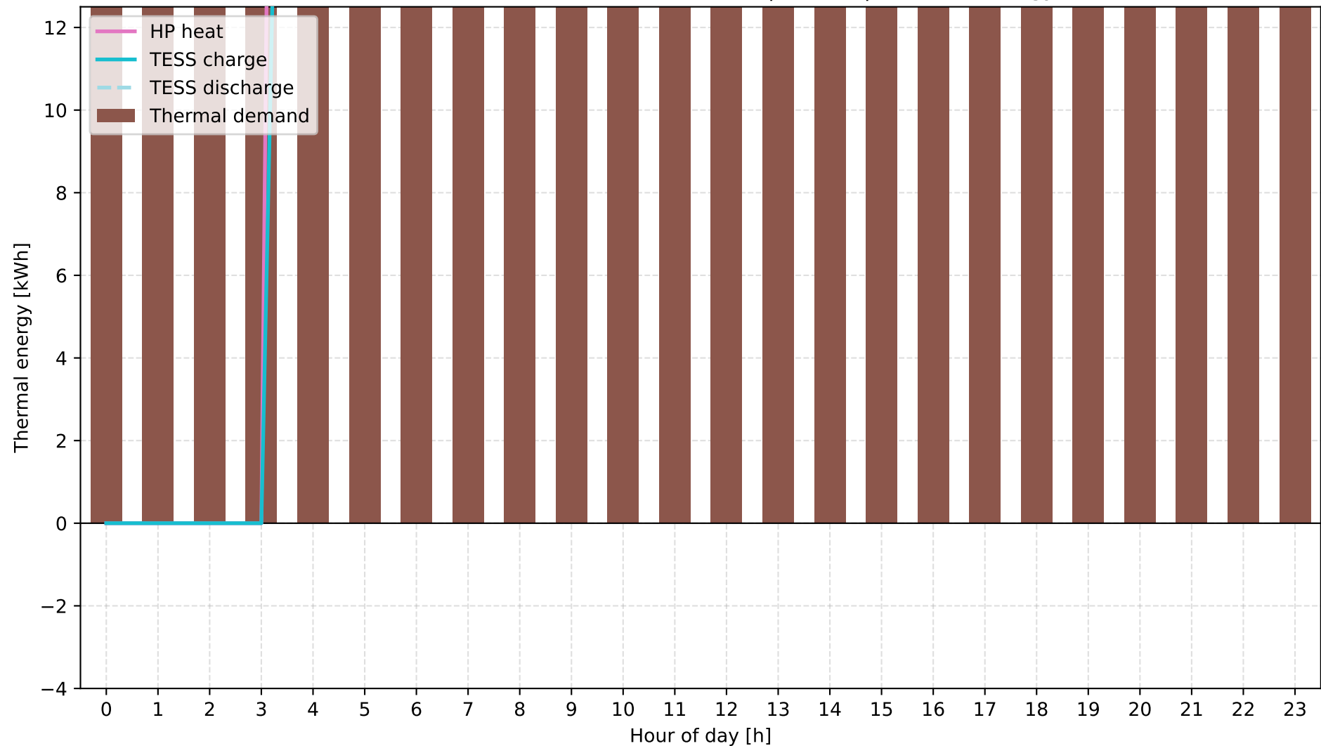
D: Grid + ASHP + PV + BESS + TESS | Winter | Thermal Energy
