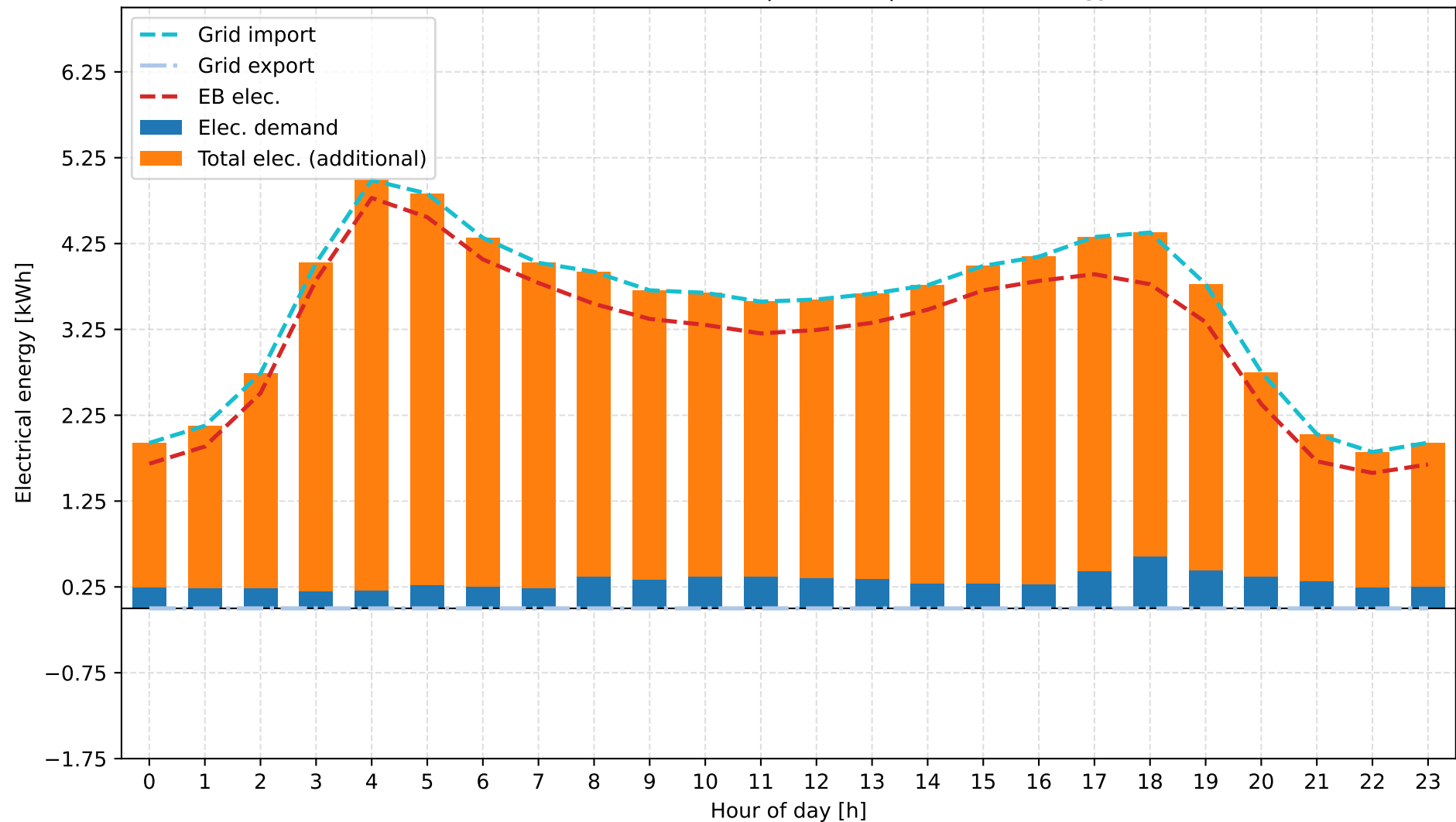
A: Grid + Electric Boiler | Autumn | Electrical Energy
