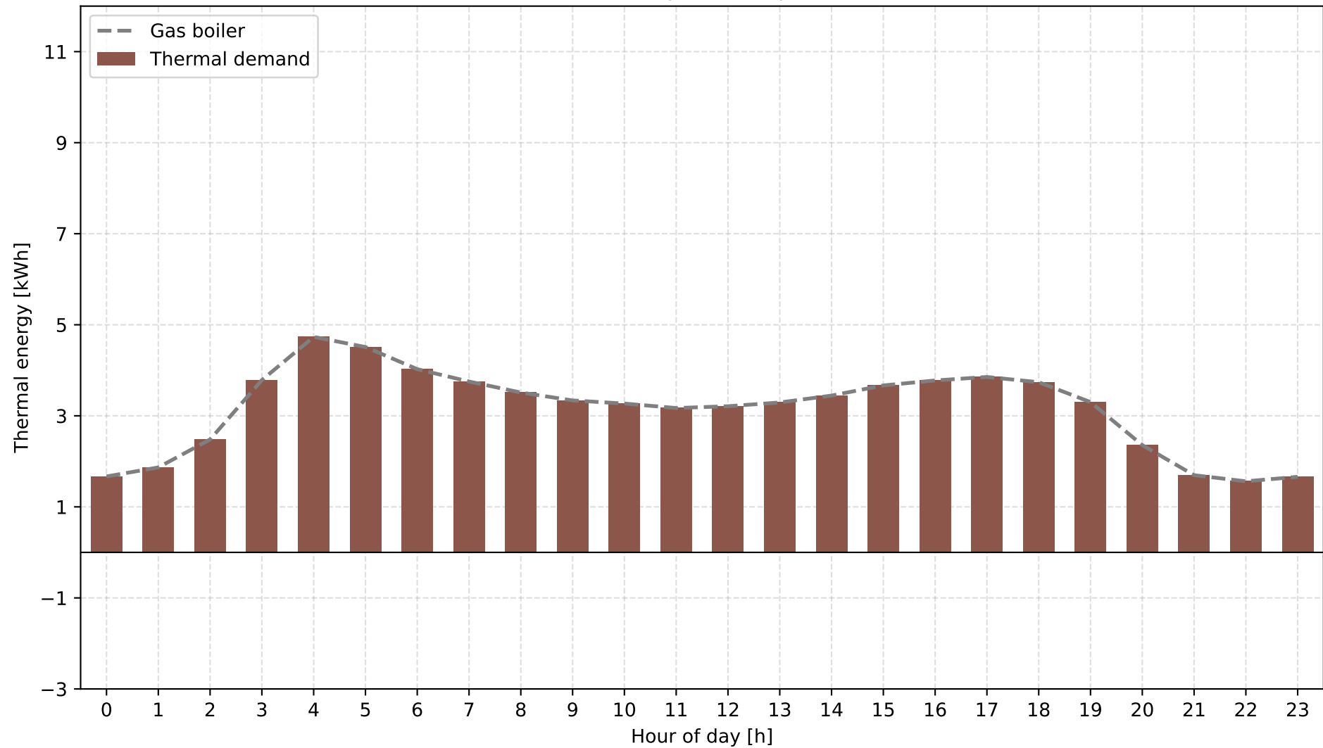
B: Grid + Gas Boiler | Autumn | Thermal Energy
