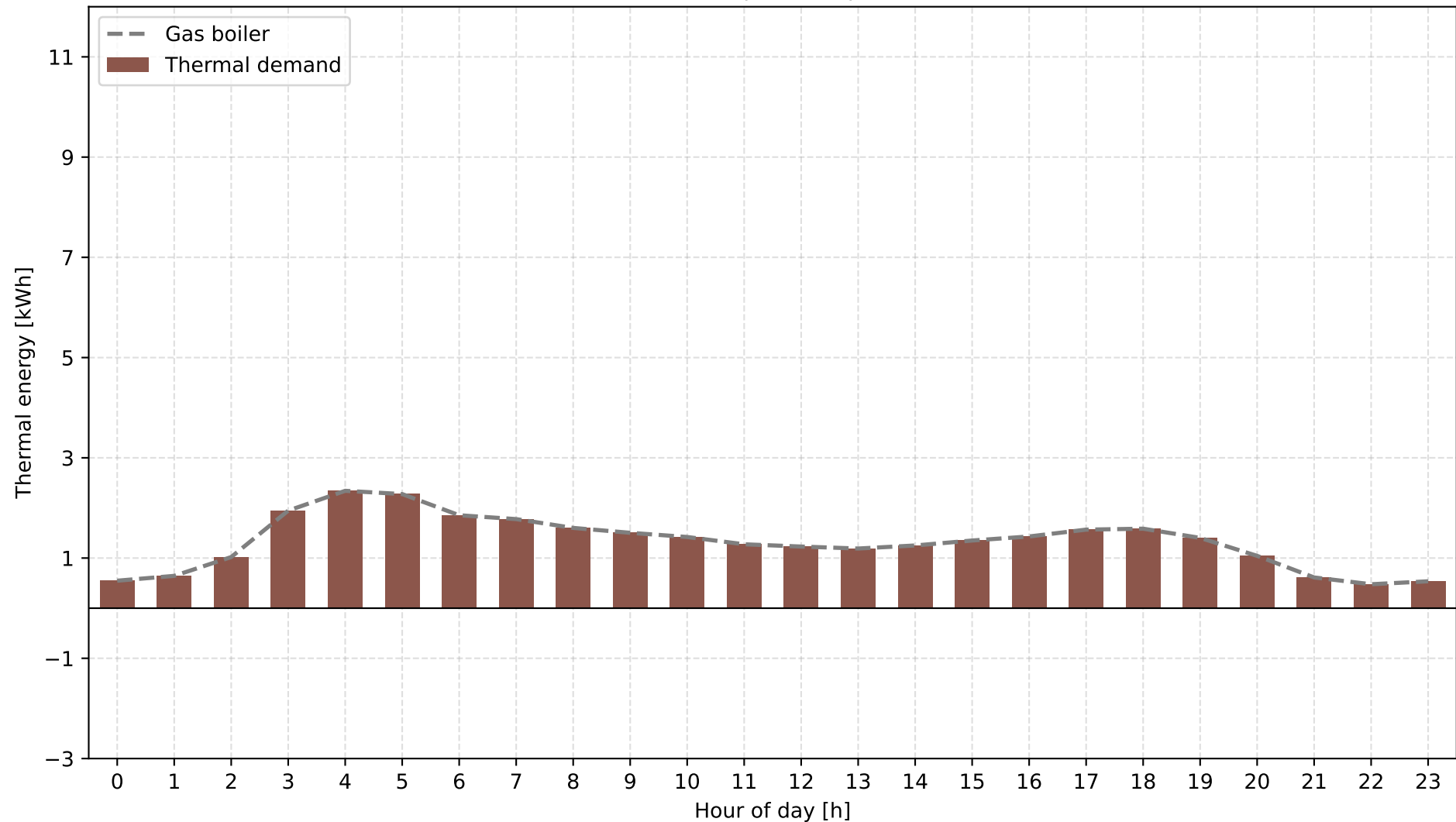
B: Grid + Gas Boiler | Spring | Thermal Energy
