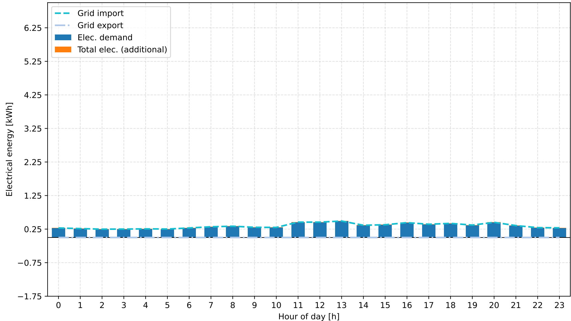
B: Grid + Gas Boiler | Summer | Electrical Energy
