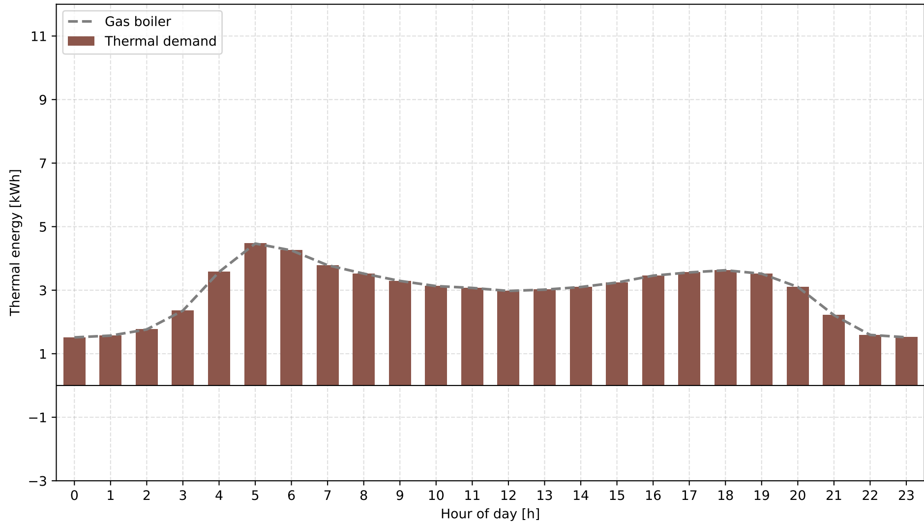
B: Grid + Gas Boiler | Winter | Thermal Energy
