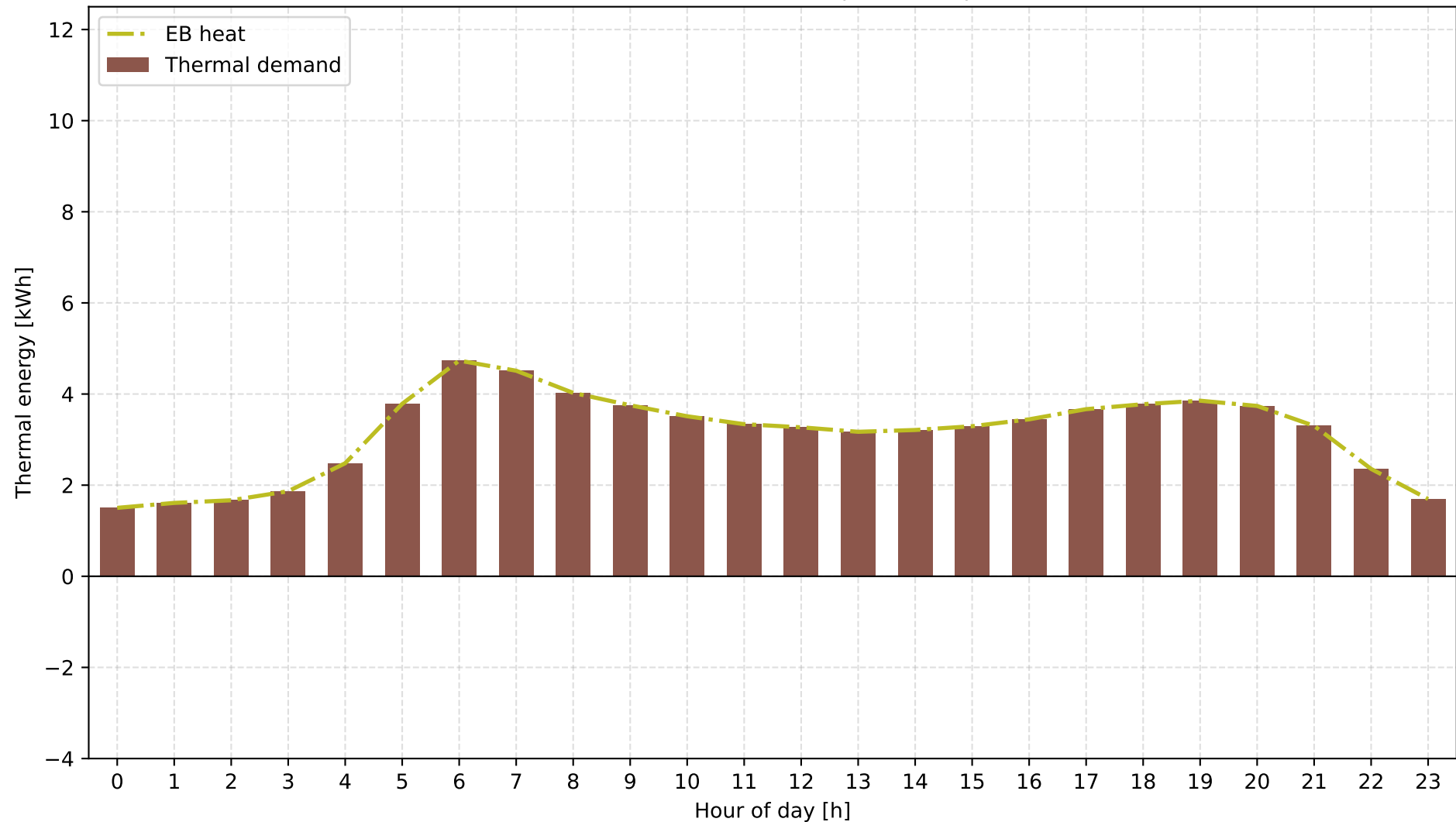
C: Grid + Electric Boiler + PV + BESS | Autumn | Thermal Energy
