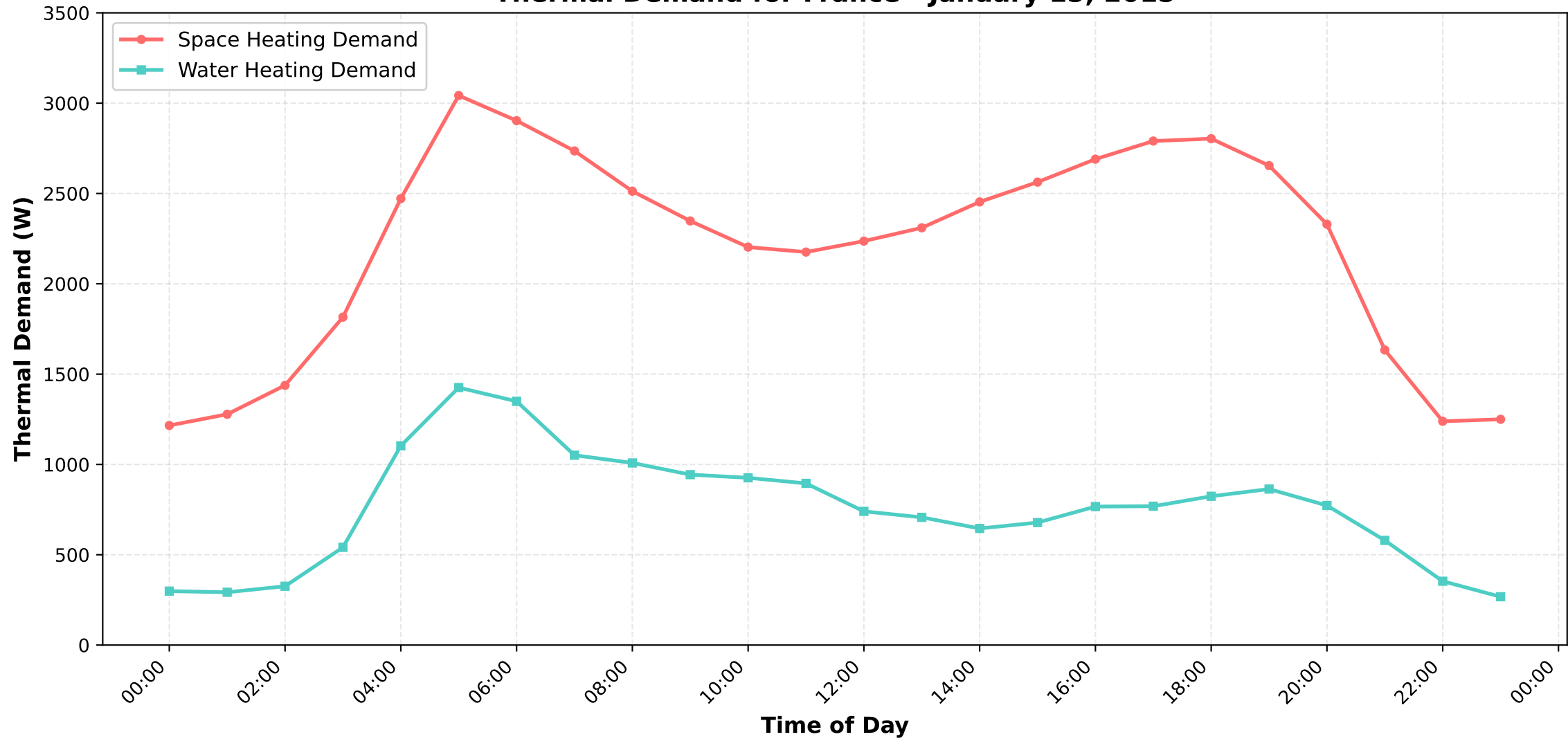
Thermal Demand for France - January 15, 2015
