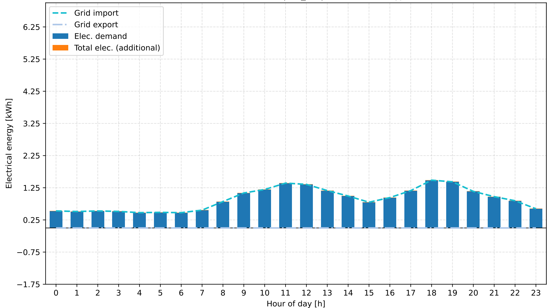
A: Grid + Gas Boiler | 15_01 | Electrical Energy
