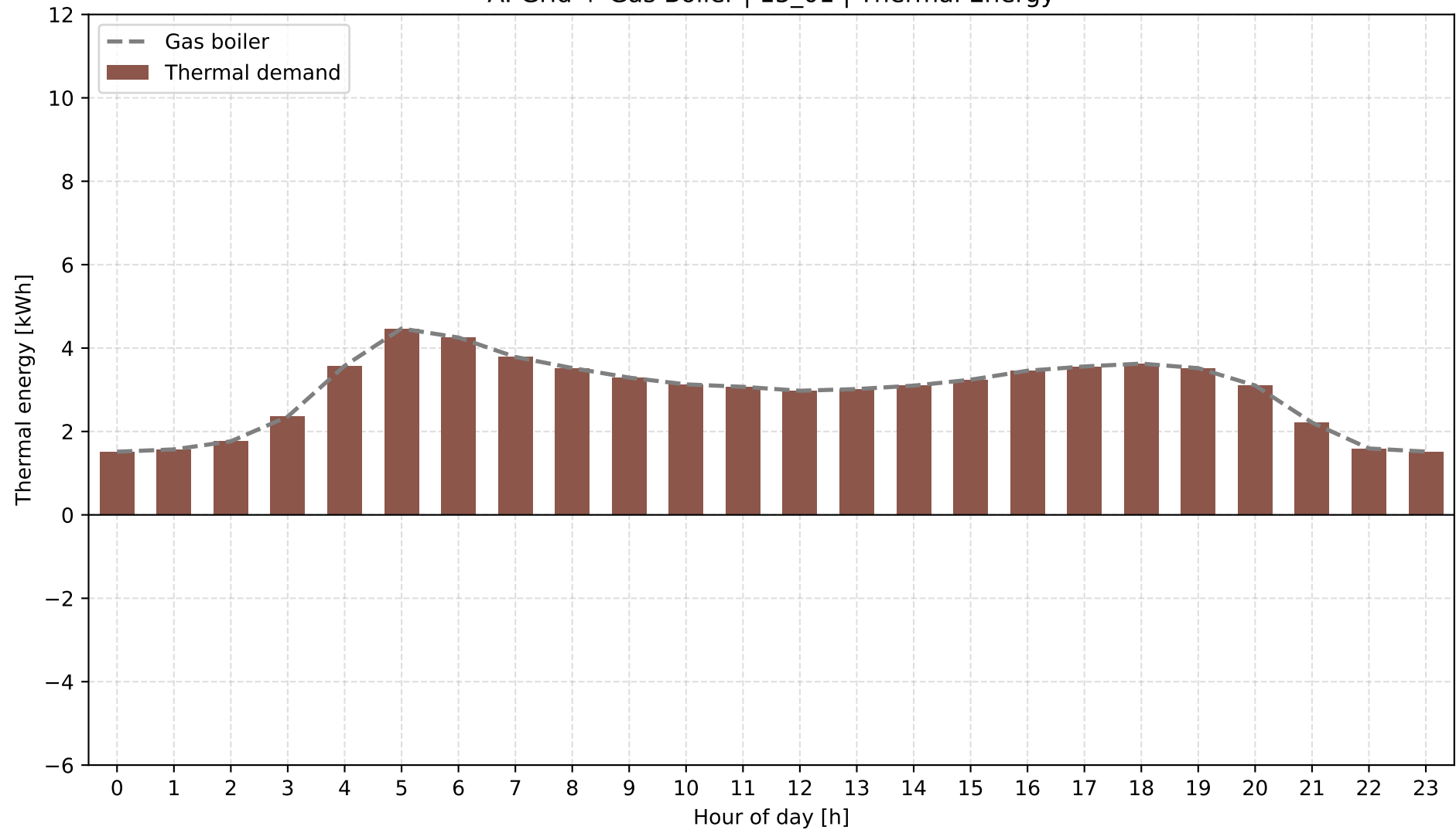
A: Grid + Gas Boiler | 15_01 | Thermal Energy
