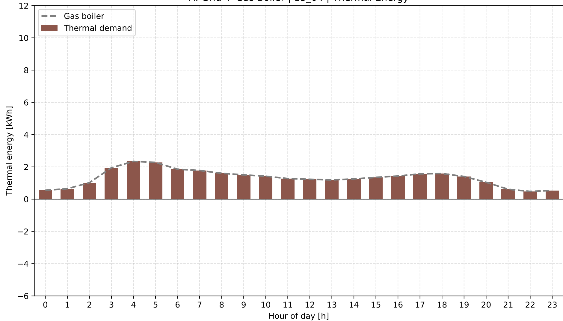
A: Grid + Gas Boiler | 15_04 | Thermal Energy
