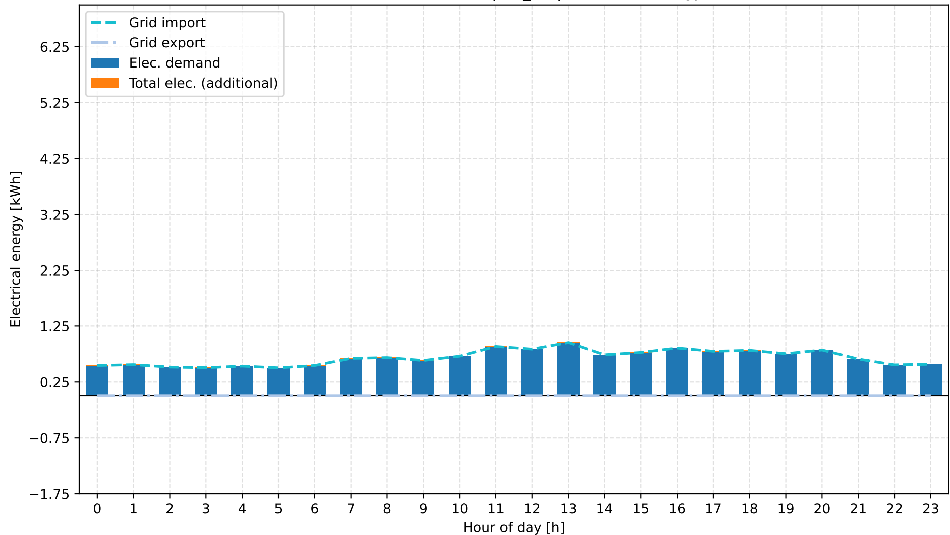
A: Grid + Gas Boiler | 15_07 | Electrical Energy
