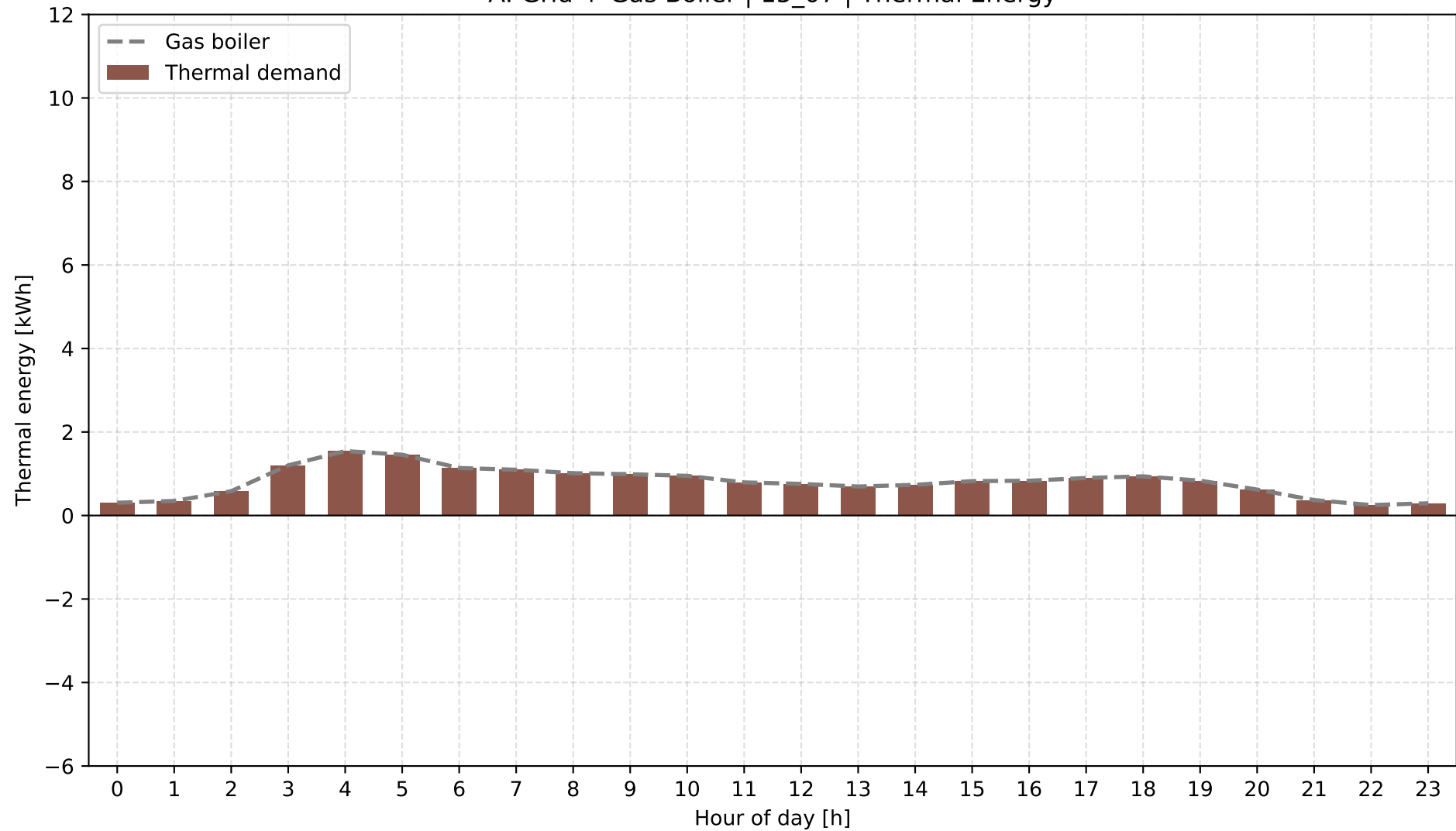
A: Grid + Gas Boiler | 15_07 | Thermal Energy
