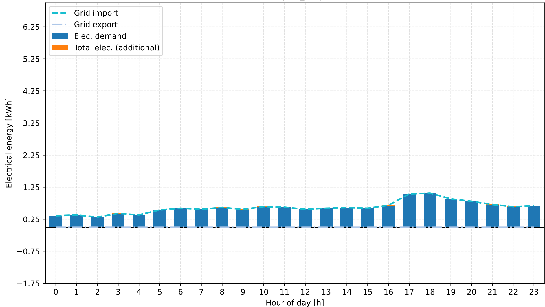
A: Grid + Gas Boiler | 15_10 | Electrical Energy
