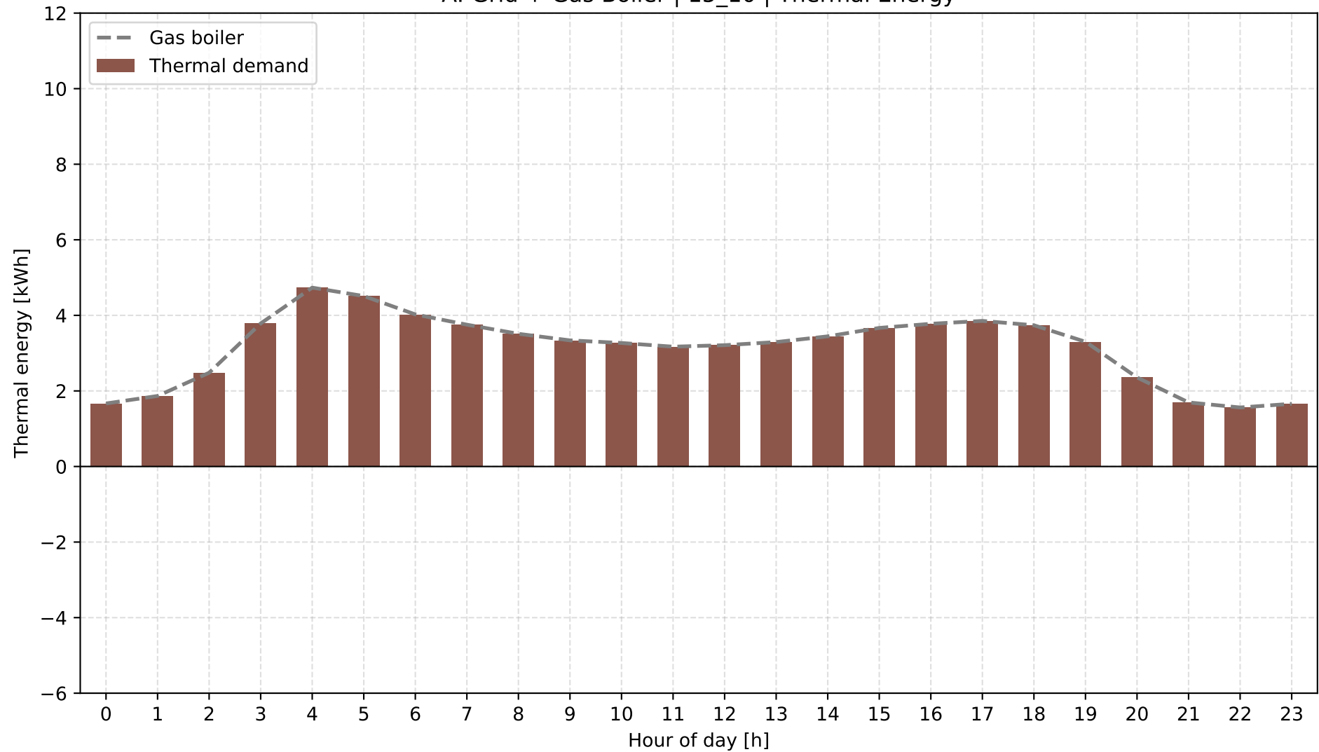
A: Grid + Gas Boiler | 15_10 | Thermal Energy
