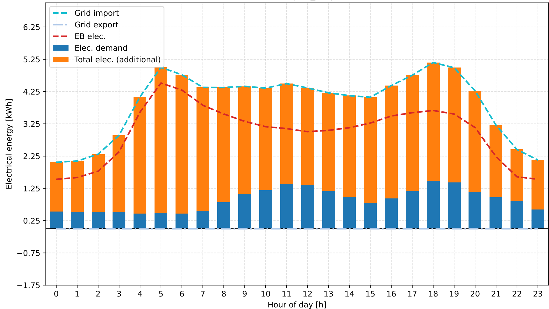
B: Grid + Electric Boiler | 15_01 | Electrical Energy
