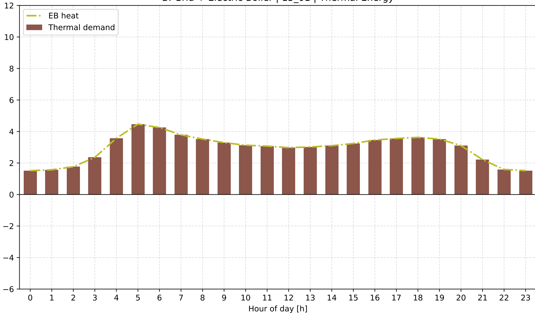
B: Grid + Electric Boiler | 15_01 | Thermal Energy
