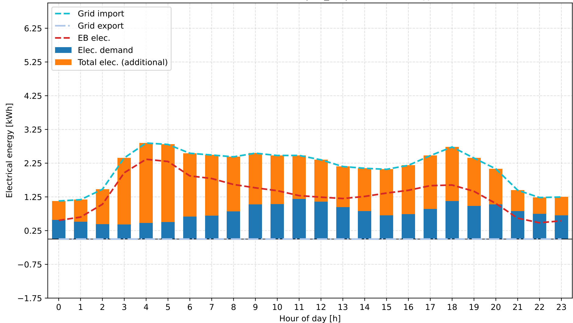
B: Grid + Electric Boiler | 15_04 | Electrical Energy
