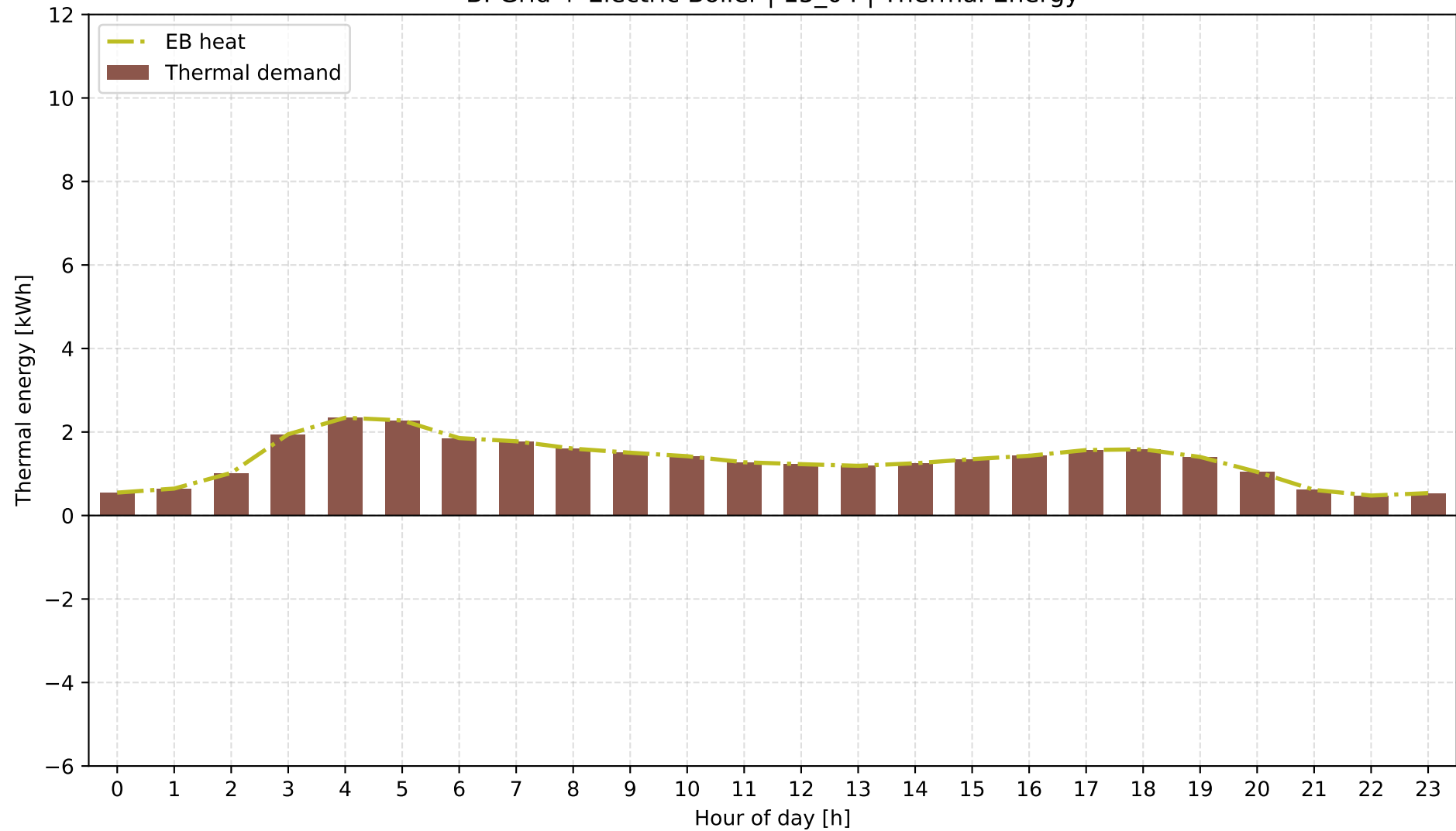
B: Grid + Electric Boiler | 15_04 | Thermal Energy
