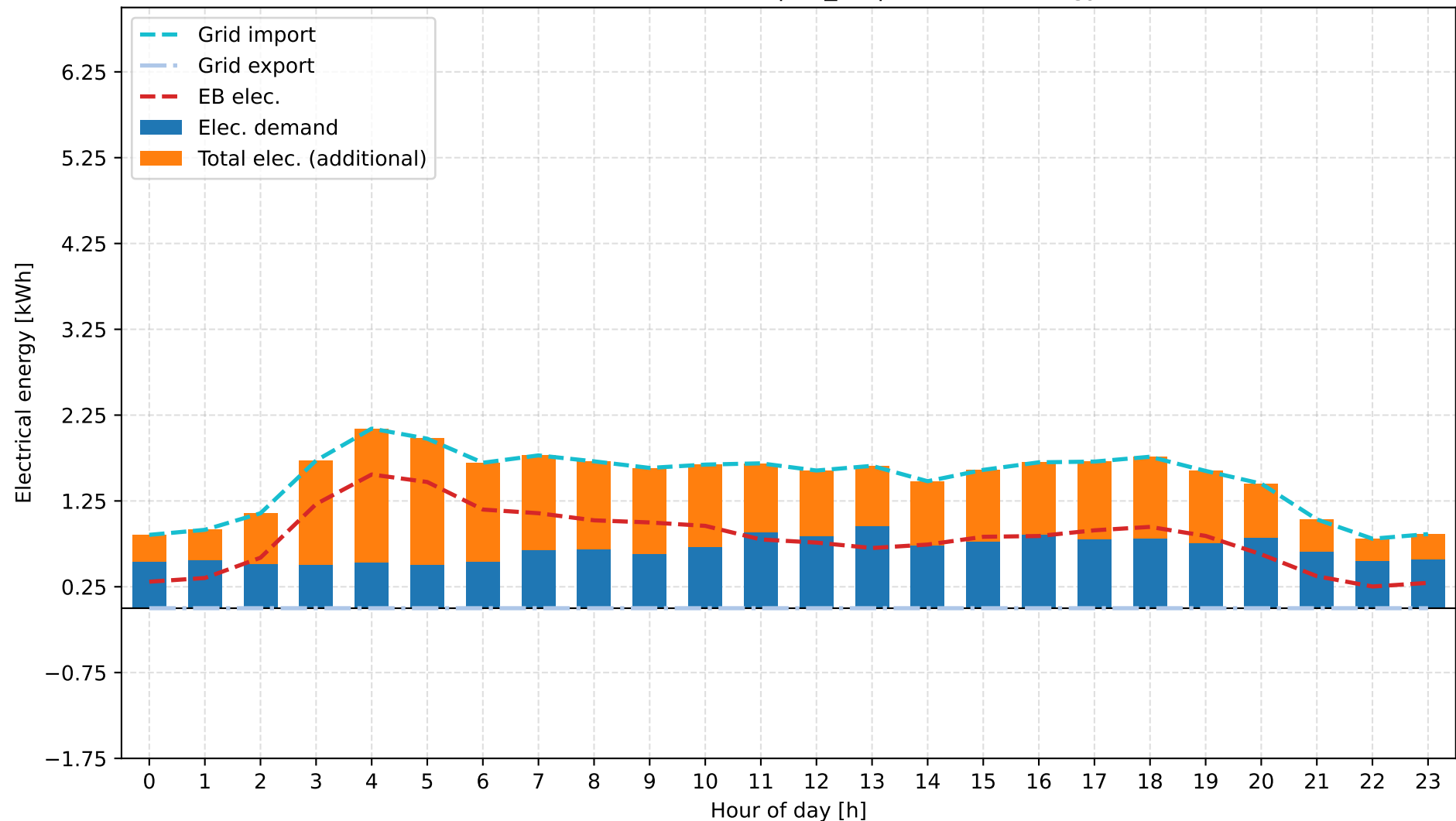
B: Grid + Electric Boiler | 15_07 | Electrical Energy
