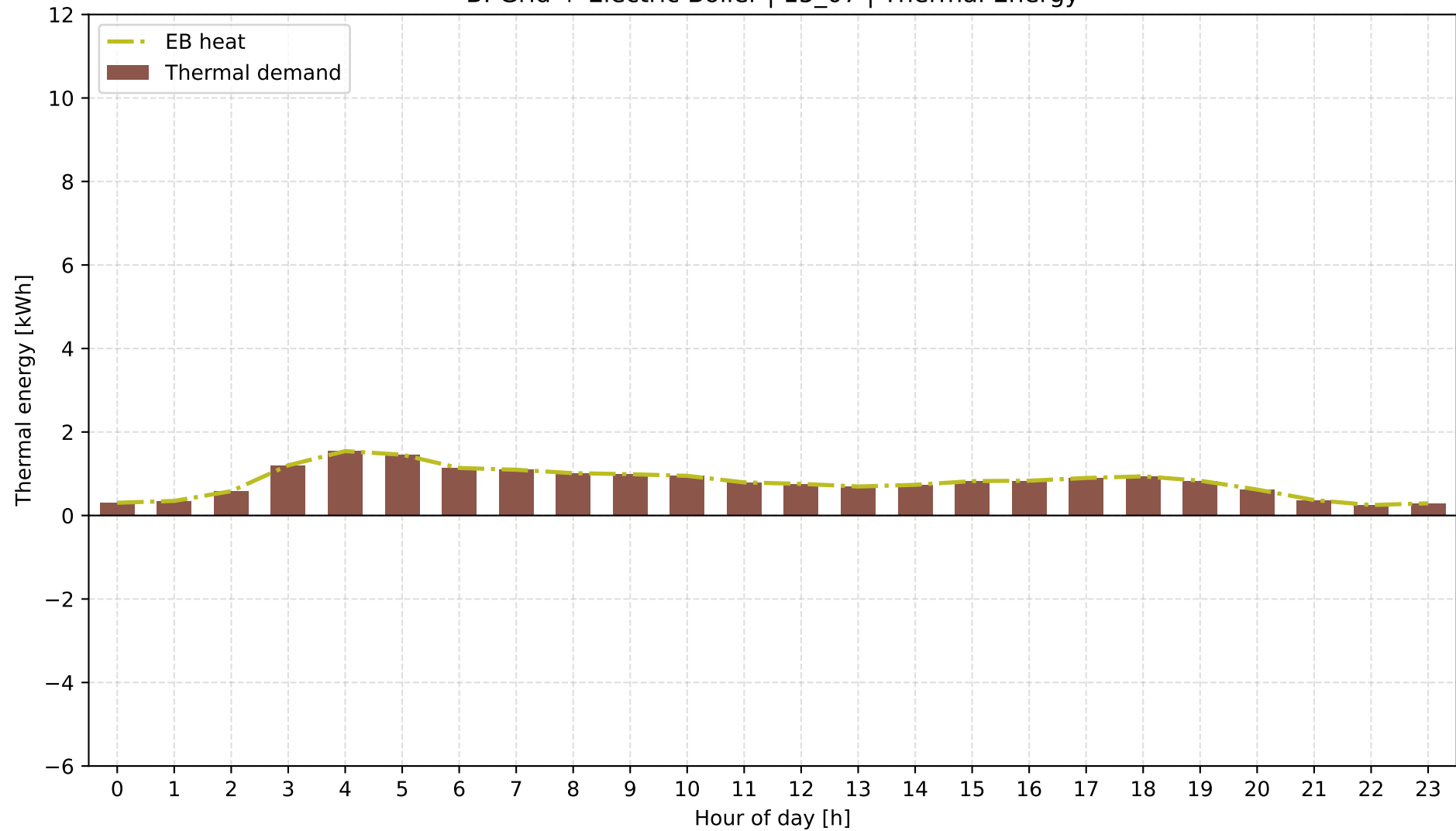
B: Grid + Electric Boiler | 15_07 | Thermal Energy
