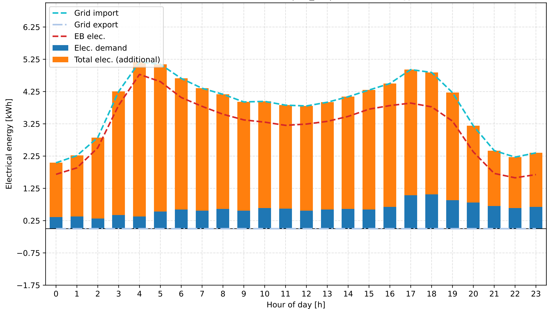
B: Grid + Electric Boiler | 15_10 | Electrical Energy
