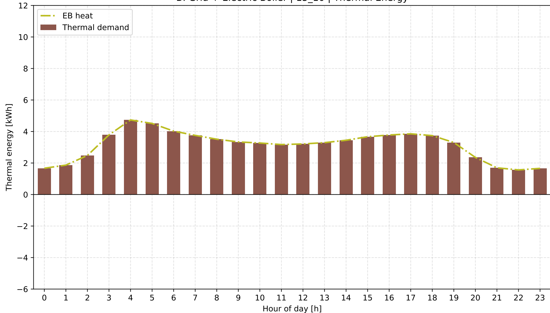
B: Grid + Electric Boiler | 15_10 | Thermal Energy
