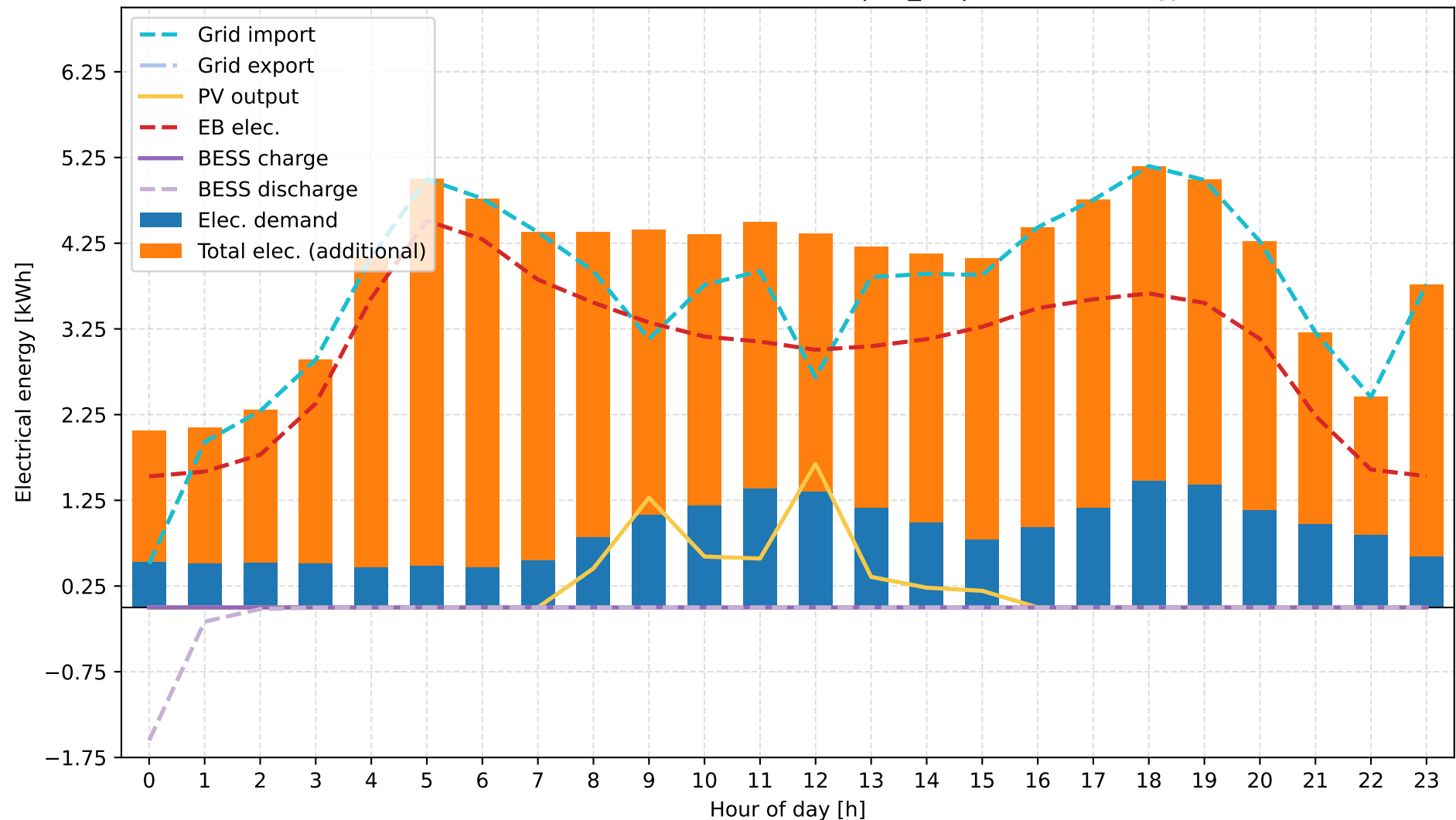
C: Grid + Electric Boiler + PV + BESS | 15_01 | Electrical Energy
