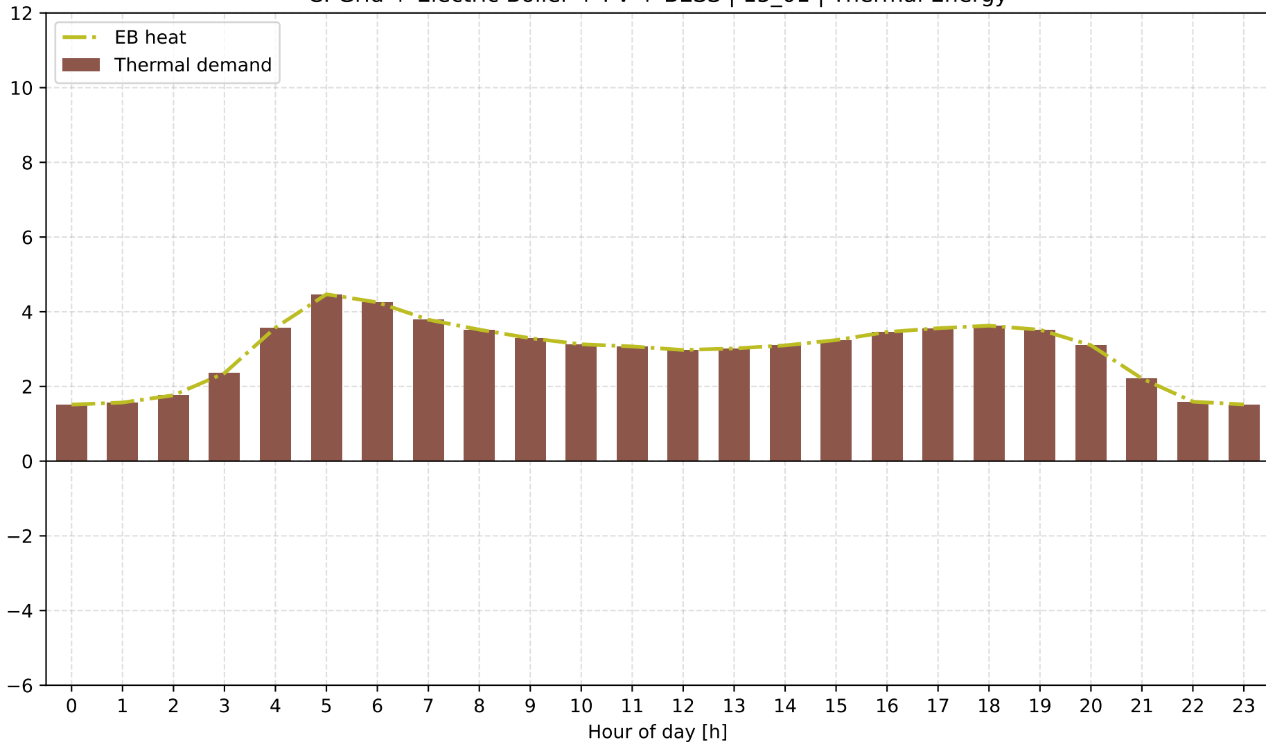
C: Grid + Electric Boiler + PV + BESS | 15_01 | Thermal Energy
