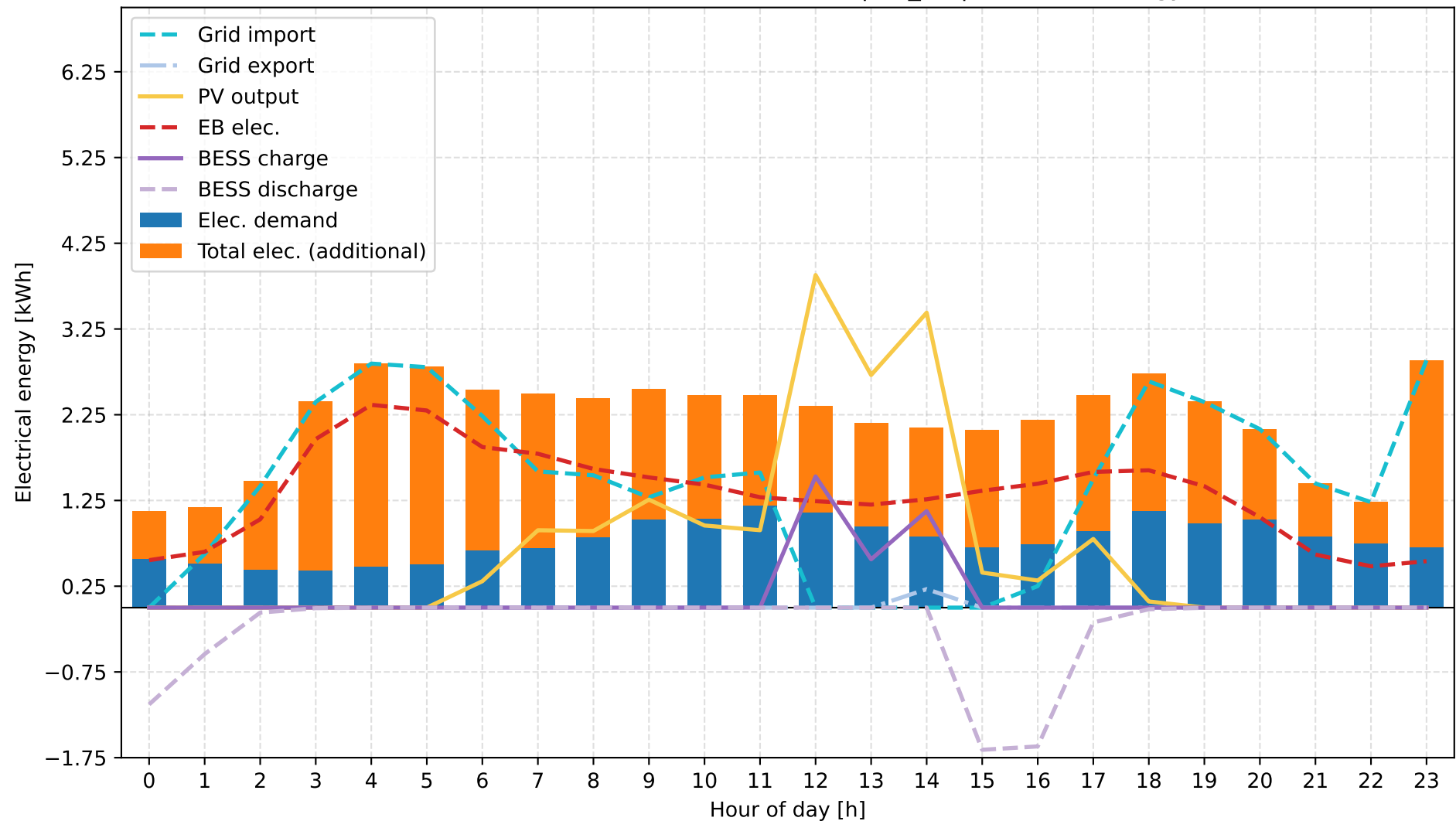
C: Grid + Electric Boiler + PV + BESS | 15_04 | Electrical Energy
