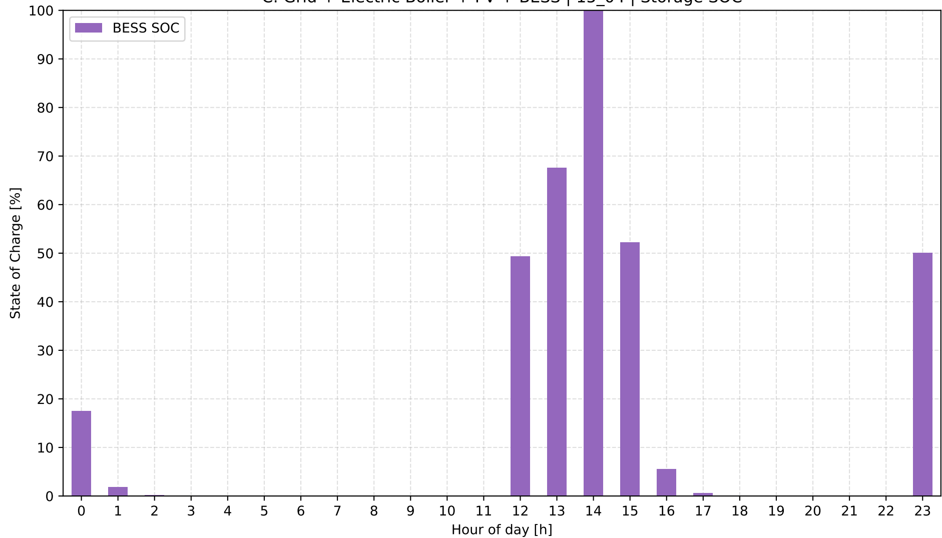
C: Grid + Electric Boiler + PV + BESS | 15_04 | Storage SOC
