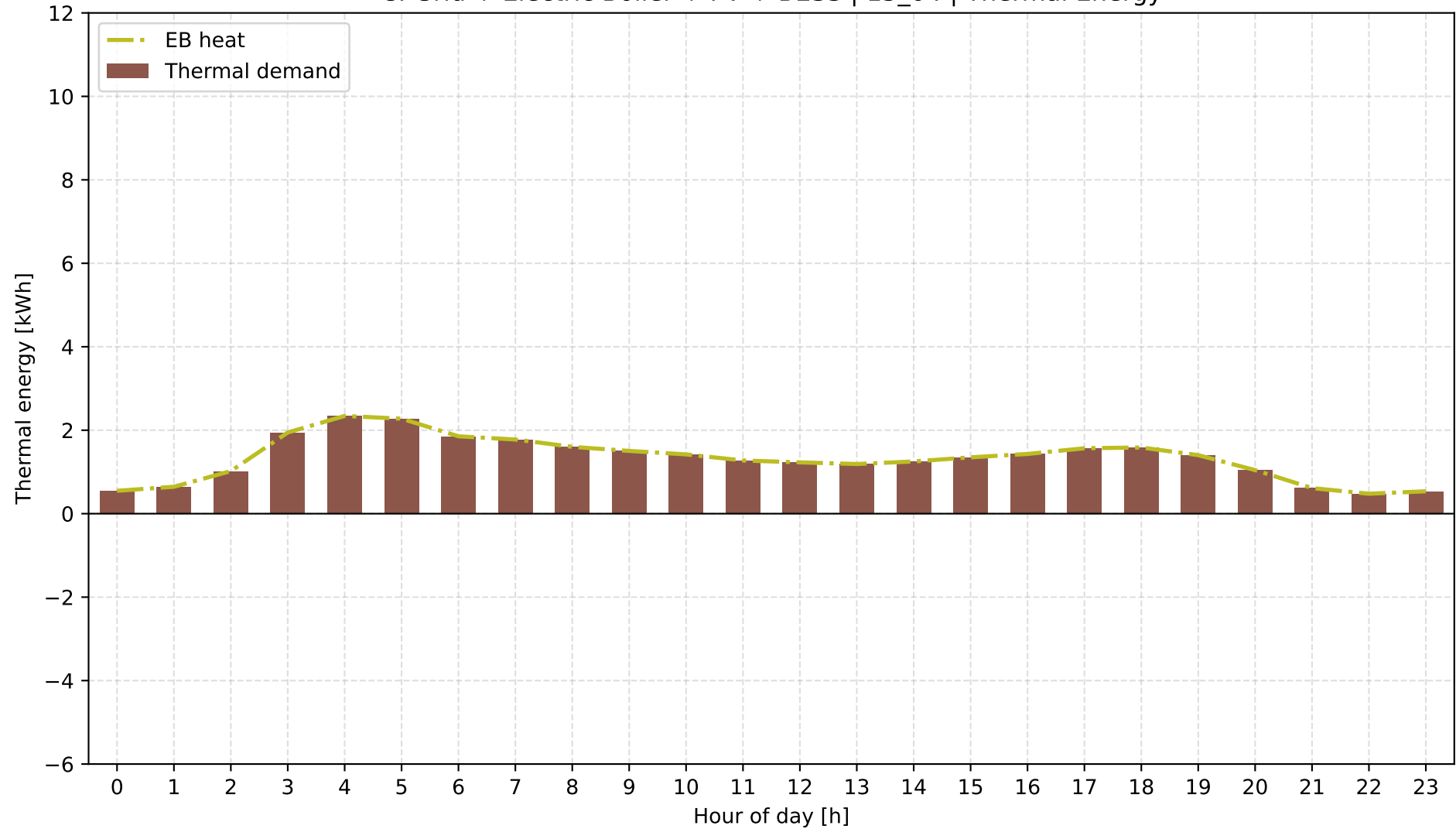
C: Grid + Electric Boiler + PV + BESS | 15_04 | Thermal Energy
