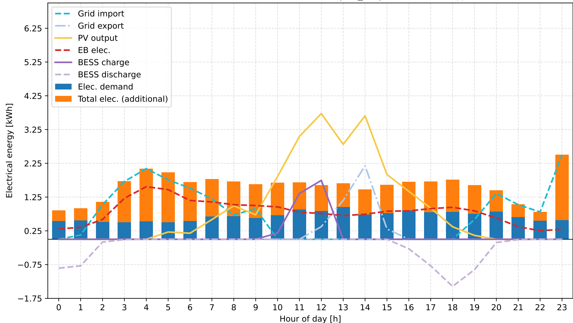
C: Grid + Electric Boiler + PV + BESS | 15_07 | Electrical Energy
