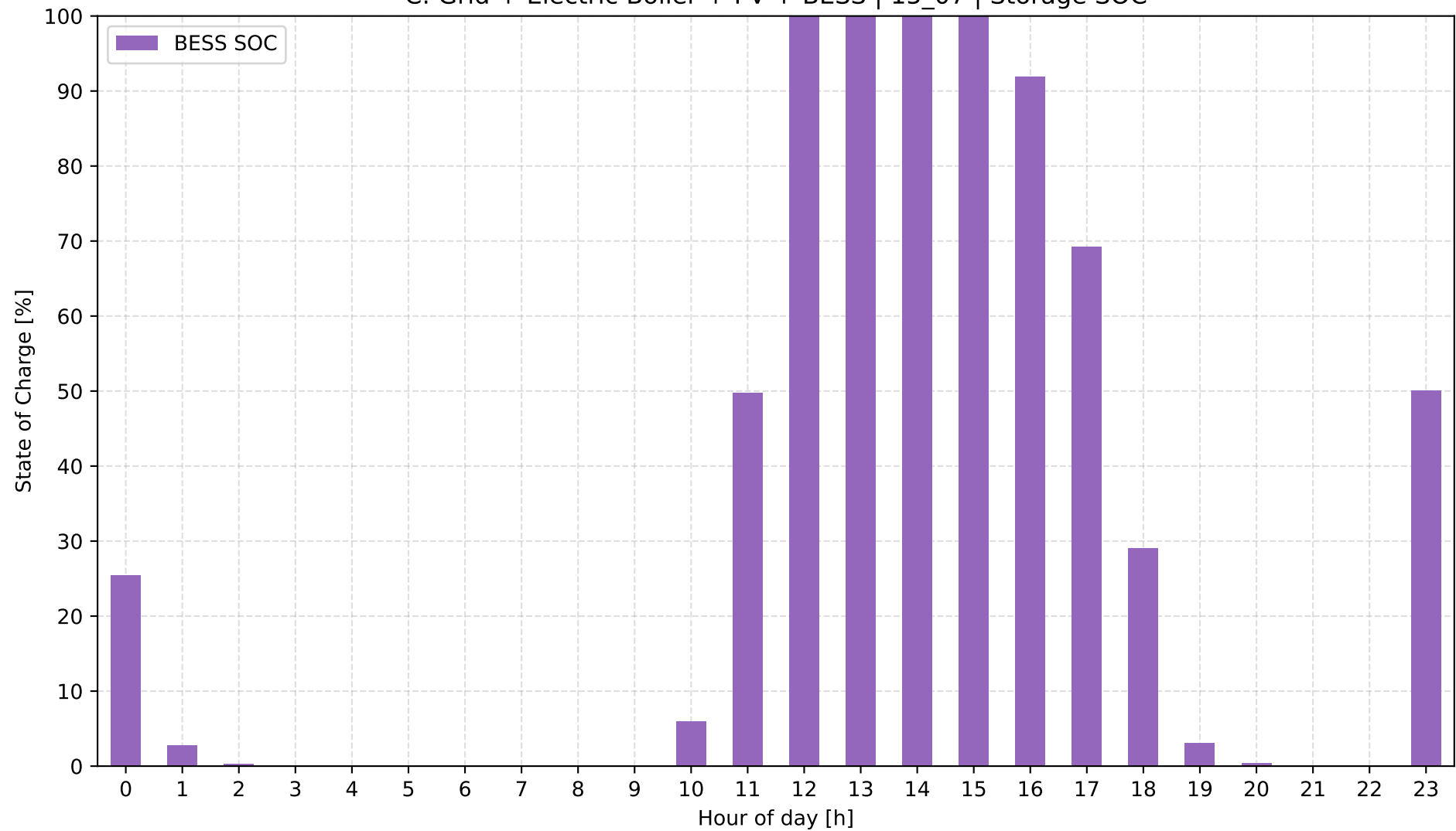
C: Grid + Electric Boiler + PV + BESS | 15_07 | Storage SOC
