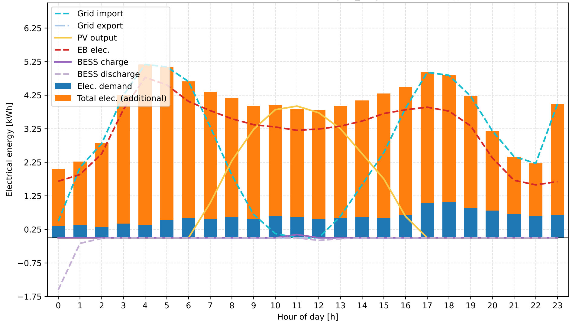
C: Grid + Electric Boiler + PV + BESS | 15_10 | Electrical Energy
