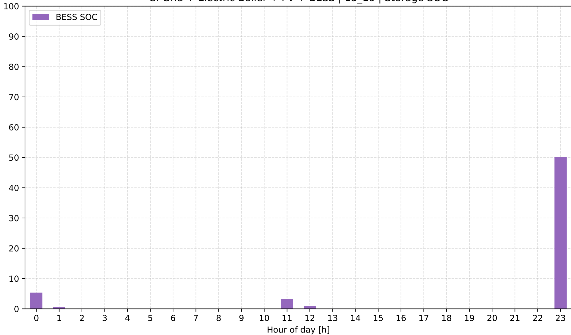
C: Grid + Electric Boiler + PV + BESS | 15_10 | Storage SOC
