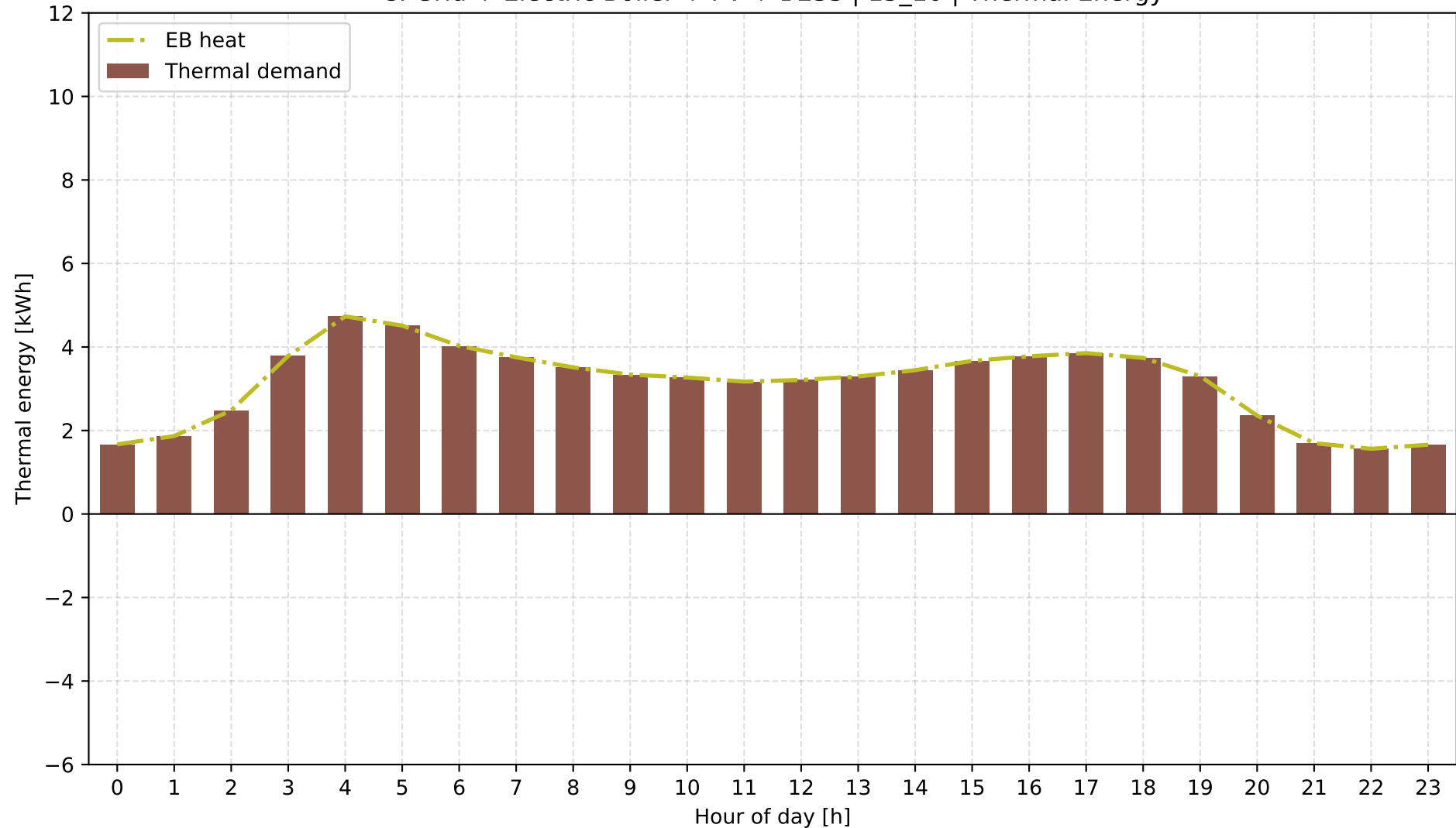
C: Grid + Electric Boiler + PV + BESS | 15_10 | Thermal Energy
