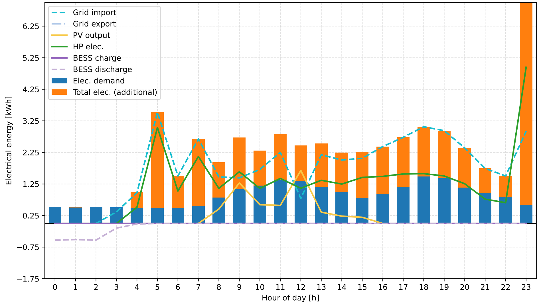
D: Grid + ASHP + PV + BESS + TESS | 15_01 | Electrical Energy
