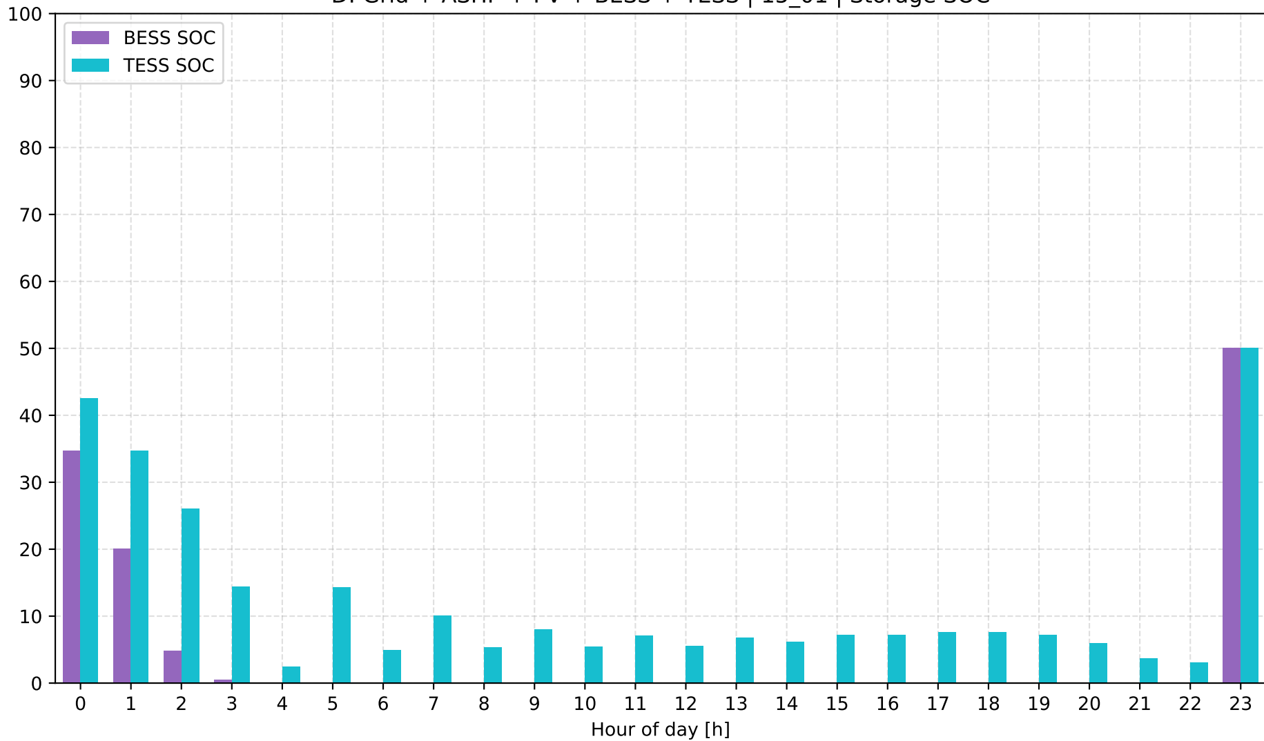
D: Grid + ASHP + PV + BESS + TESS | 15_01 | Storage SOC
