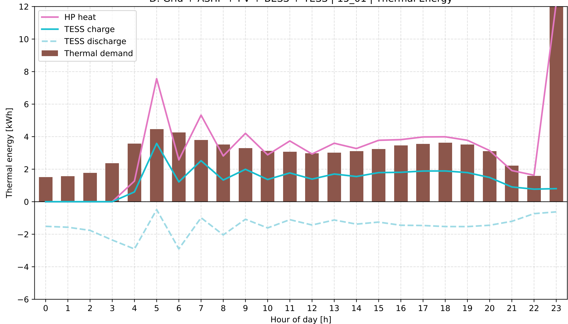
D: Grid + ASHP + PV + BESS + TESS | 15_01 | Thermal Energy
