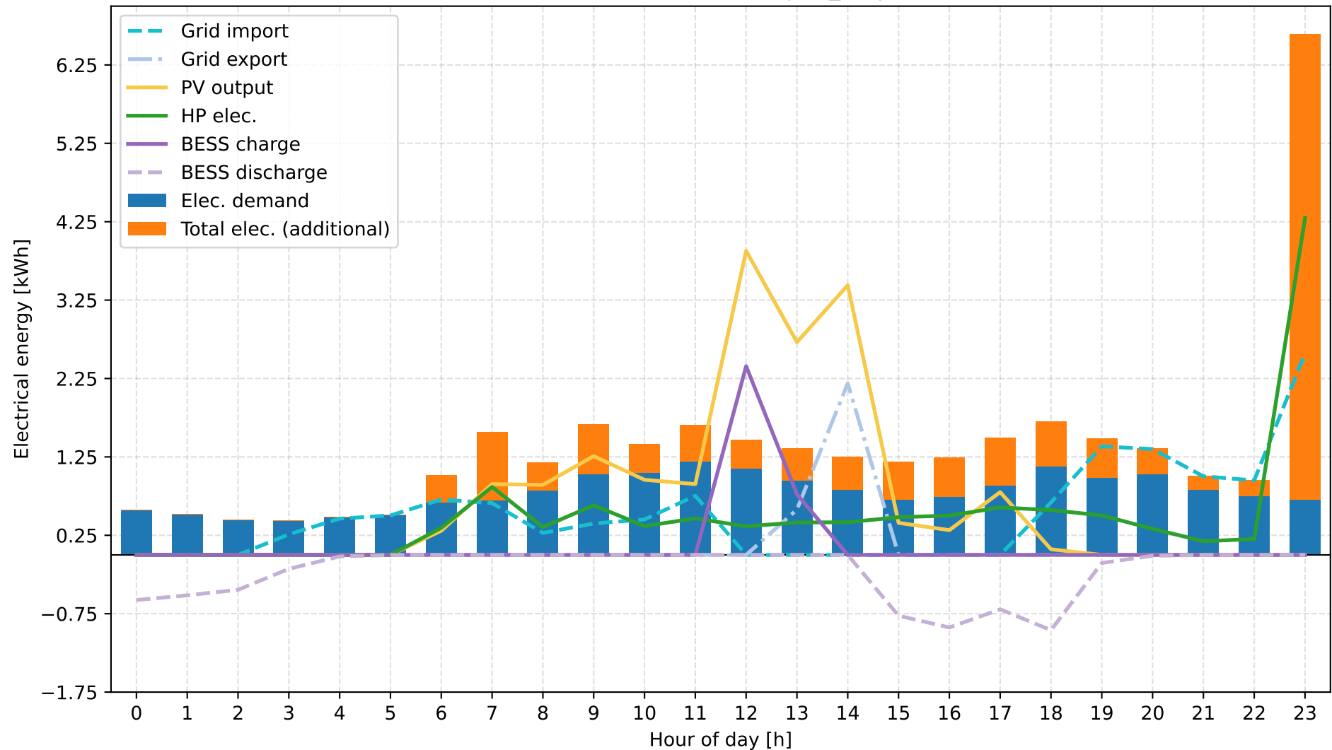
D: Grid + ASHP + PV + BESS + TESS | 15_04 | Electrical Energy
