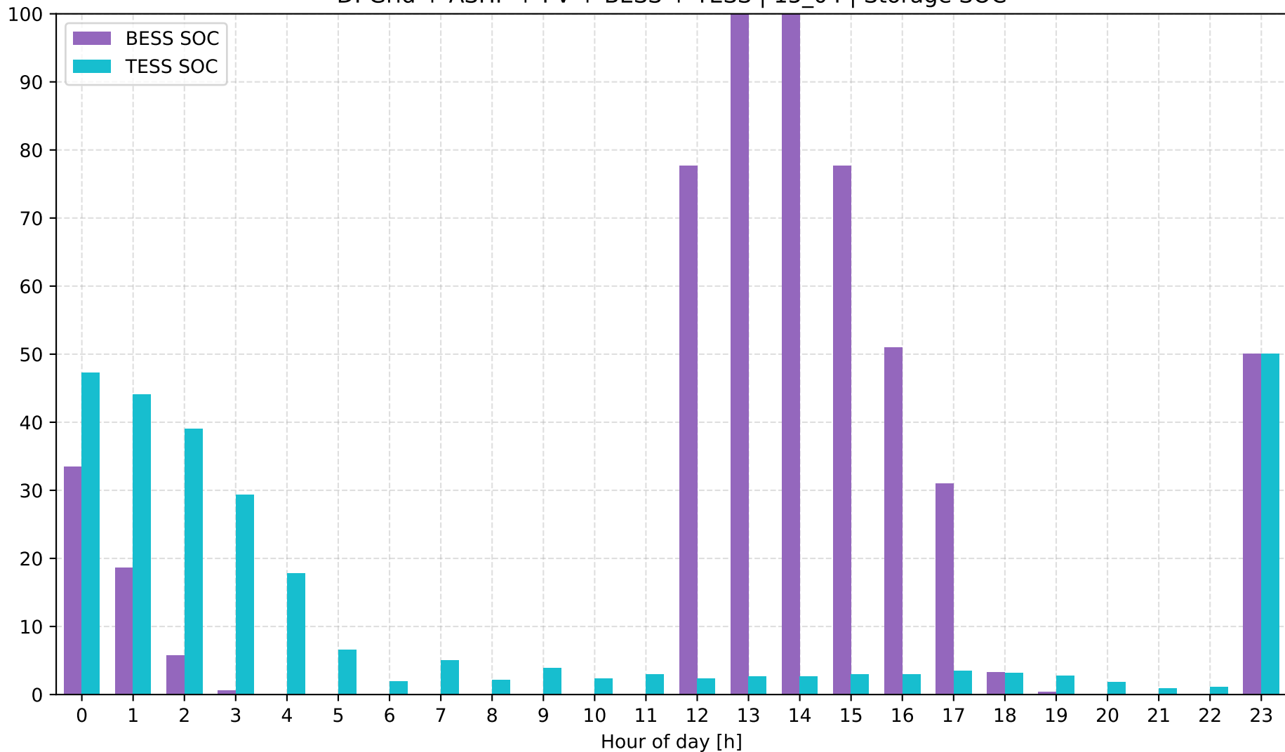
D: Grid + ASHP + PV + BESS + TESS | 15_04 | Storage SOC
