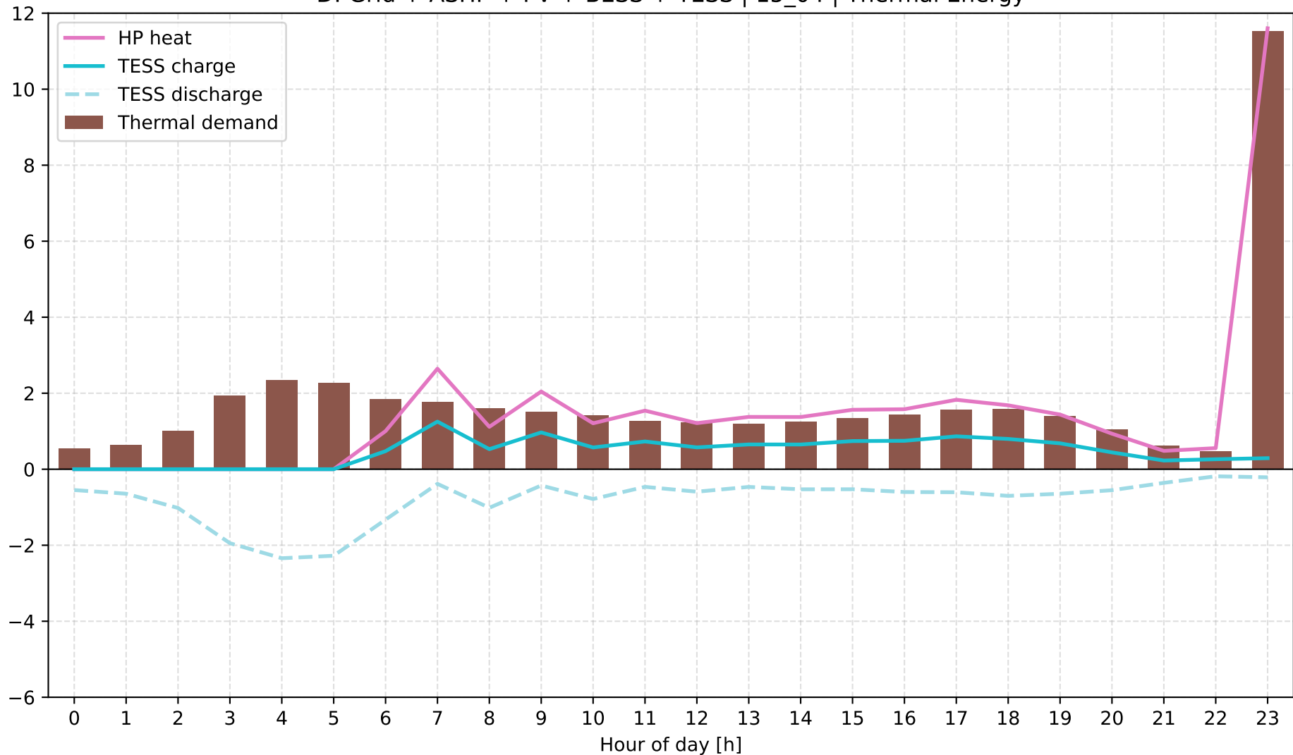
D: Grid + ASHP + PV + BESS + TESS | 15_04 | Thermal Energy
