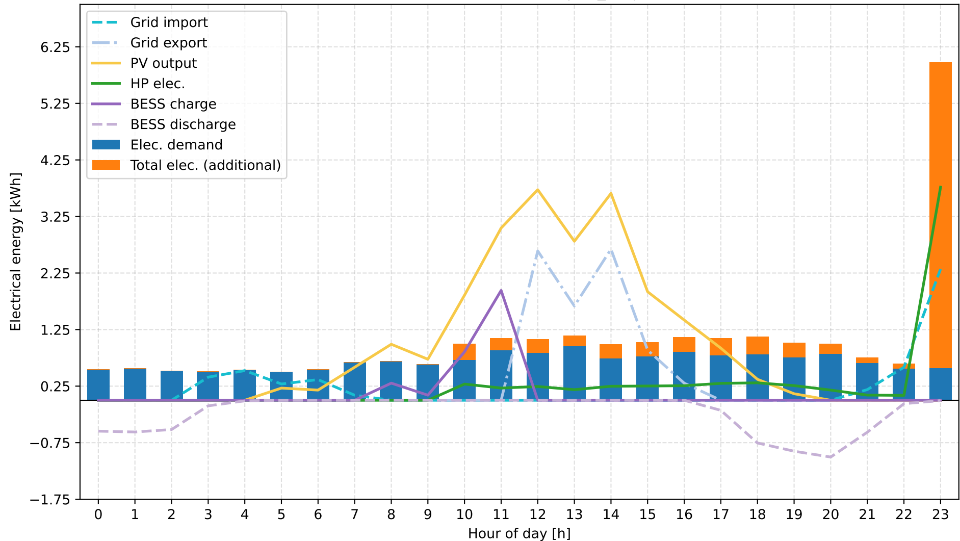
D: Grid + ASHP + PV + BESS + TESS | 15_07 | Electrical Energy
